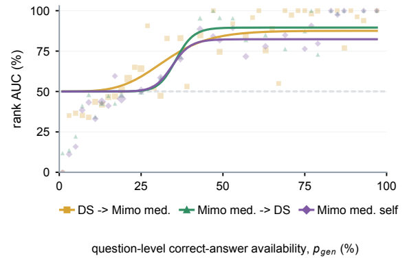
b HLE multiple choice: medium-thinking pairs
