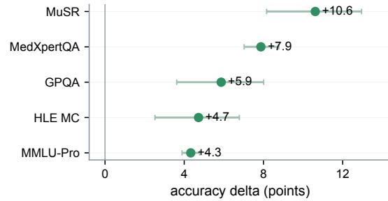
Extended Data Fig. 4 | Fixed-pool gains vary by benchmark and correct-answer availability a , Coverage of the offline comparison that reused stored candidates and judge orderings without new model calls. DeepSeek-V4-Flash (Preview, medium-thinking) generated and ranked five pools of eight candidates ( k = 8 ) per question, yielding 16,278 questions and 81,390 pools. The judge returned a usable complete ordering for every retained pool; no question was lost because of a missing or invalid ranking response. b , Question-level accuracy for one candidate sampled from the full bank, a control that randomly shuffles the judge's order, majority vote over the stored pool and selection of the judge's first-ranked candidate. Results are shown across five benchmarks using the same offline candidate pools. Bars are point estimates; paired uncertainty is shown in c . c , Change in accuracy when first-ranked selection replaced majority vote on the same candidate pools. Points are mean paired question-level differences by benchmark and bars are conditional 95% CIs from 1,000 question bootstraps. All five estimates are positive. d , Gain over one candidate sampled from the full bank across nine bins of p_{gen} , the question-level correct fraction in that bank. Curves show majority vote, the shuffled-order control and first-ranked selection. Values are descriptive binned point estimates rather than fitted thresholds or universal availability ranges. Source data are provided with this paper.
