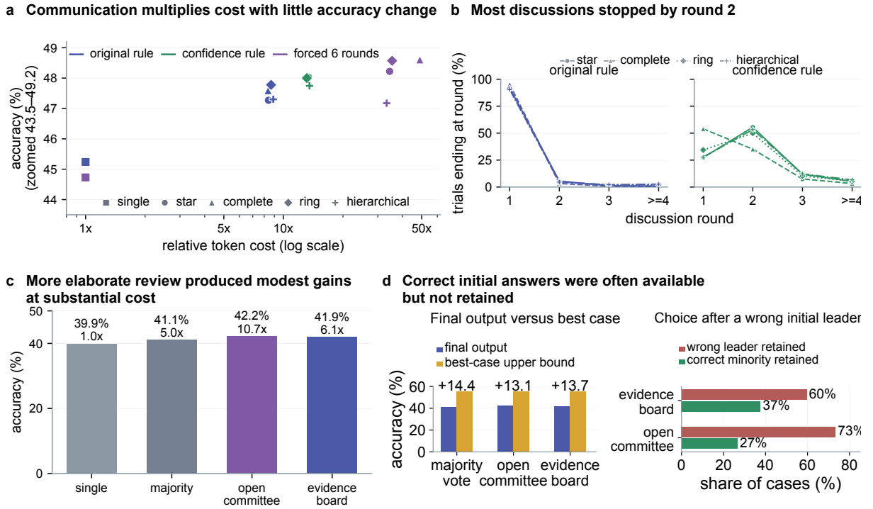
Extended Data Fig. 1 | Initial multi-agent experiments show costly communication and loss of available correct answers a , Initial comparison of four five-agent communication layouts ( n = 3,150 trials per layout and stopping condition). The original consensus rule allowed early stopping; a confidence-qualified rule required sufficiently confident agreement; and forced-six-round execution disabled early stopping. Star, complete, ring and hierarchical layouts produced similar accuracy, while token cost rose from about 8-9x with the original rule to 33-49x when all six rounds were required. b , Stopping-round distributions by communication layout. The original early-stopping rule ended 90.48-95.37% of trials after round 1; even when stopping required confidence-qualified agreement, 81.11-89.17% ended by round 2. Rounds 4-10 are pooled. Forced-six-round runs are omitted because round 6 was imposed by design. c , Protocol comparison repeated with three random seeds ( n = 7,350 cases per protocol). The single-answer protocol produced one independently generated response. Majority vote chose the most common of five independently generated answers. In the open committee, five agents answered independently and then answered again after reviewing source-labelled responses from the other four agents. The anonymous evidence board pooled evidence from five independent responses without peer review and removed source labels and explicit links between evidence statements and answer options. Answer-selection details are provided in Methods. Accuracy ranged from 39.88% for the single-answer protocol to 42.20% for the open committee, while token cost ranged from 1.00x to 10.73x. d , Answer-selection analysis ( n = 7,350 per condition). An oracle that counted a case as correct whenever any initial answer was correct exceeded the actual final output by 13.13-14.38 points. When the most common initial answer was wrong but a less frequent correct answer was present, both multi-agent review conditions still selected the most frequent incorrect answer more often than the less frequent correct answer. Source data are provided with this paper.
