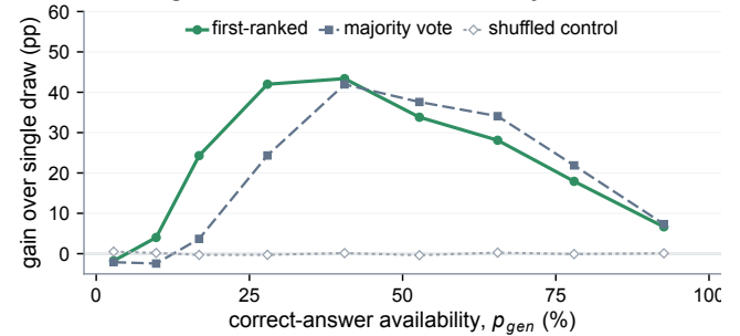
Extended Data Fig. 4 | Fixed-pool gains vary by benchmark and correct-answer availability a , Coverage of the offline comparison that reused stored candidates and judge orderings without new model calls. DeepSeek-V4-Flash (Preview, medium-thinking) generated and ranked five pools of eight candidates ( k = 8 ) per question, yielding 16,278 questions and 81,390 pools. The judge returned a usable complete ordering for every retained pool; no question was lost because of a missing or invalid ranking response. b , Question-level accuracy for one candidate sampled from the full bank, a control that randomly shuffles the judge's order, majority vote over the stored pool and selection of the judge's first-ranked candidate. Results are shown across five benchmarks using the same offline candidate pools. Bars are point estimates; paired uncertainty is shown in c . c , Change in accuracy when first-ranked selection replaced majority vote on the same candidate pools. Points are mean paired question-level differences by benchmark and bars are conditional 95% CIs from 1,000 question bootstraps. All five estimates are positive. d , Gain over one candidate sampled from the full bank across nine bins of p_{gen} , the question-level correct fraction in that bank. Curves show majority vote, the shuffled-order control and first-ranked selection. Values are descriptive binned point estimates rather than fitted thresholds or universal availability ranges. Source data are provided with this paper.
