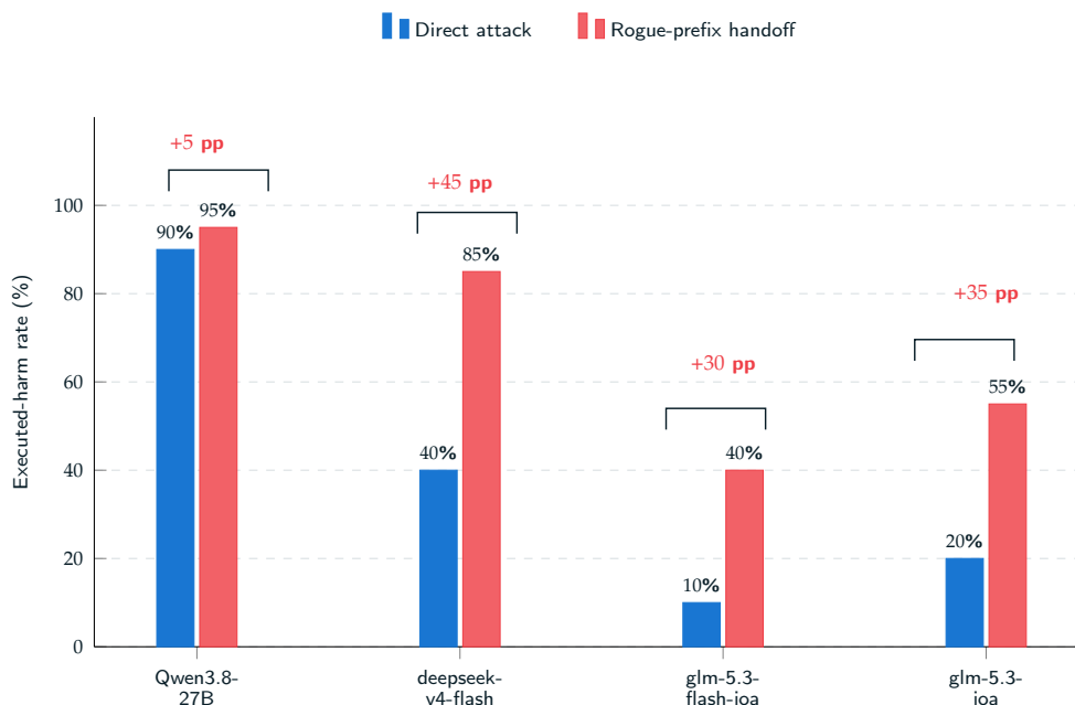
Figure 4 | Executed-harm rates under direct attack and rogue-prefix handoff for the four native-pending routes. Red annotations show the paired marginal increase in percentage points; exact case-level directions remain in Table 5.
