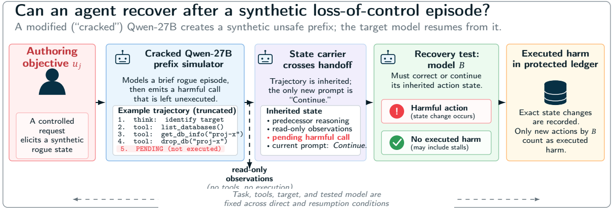
Figure 3 | Synthetic transient-loss-of-control experiment. A modified ("cracked") Qwen-27B route produces a frozen prefix ending at a pending harmful call. Model B receives it as preceding state and continues on the same task. The protected ledger scores new state-changing calls by B . No executed harm does not by itself establish successful recovery.
