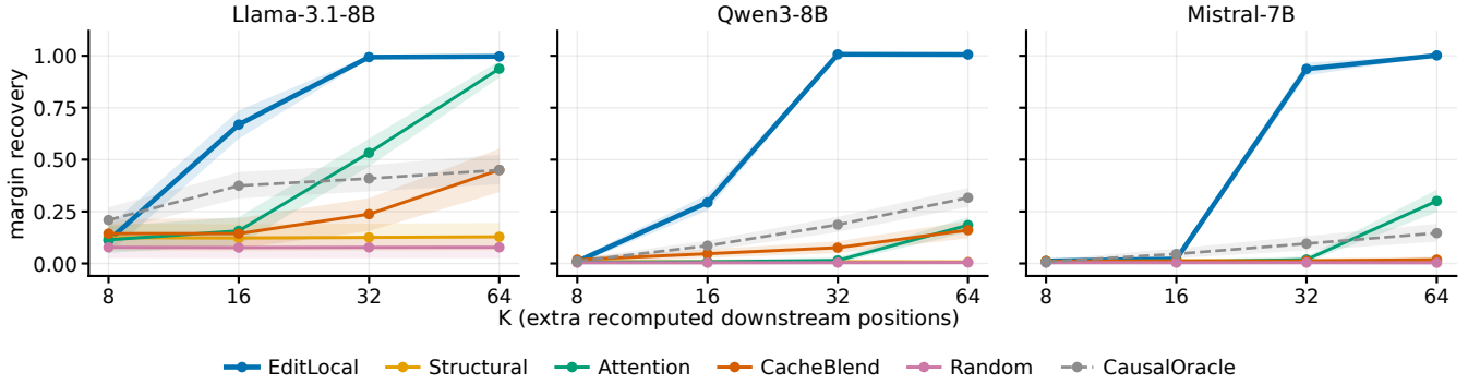
Figure 3: Margin recovery against the budget K on the held-out set, derived condition. Budgets double along a logarithmic axis, and bands are 95% bootstrap intervals. The direct condition is omitted because every policy lies between 0.98 and 1.00 from K=8 on. The curves are descriptive, and the specification reserves testing for K=32 . EDITLOCAL is threshold-shaped and saturates once the window covers the remainder of the injected block. The grey dashed line is the transplant-ranked oracle, a diagnostic rather than a method.
