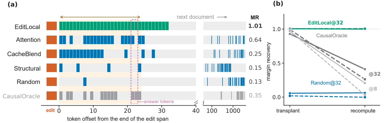
Figure 2: Contiguity, not localization, decides repair. (a) Selections for a representative held-out Llama item at K=32 . Orange marks the edit span, repaired outside the budget, and grey marks states left stale. Only EDITLOCAL forms an unbroken path from the edit through the answer. (b) Margin recovery under transplant and recomputation on identical sets from 15 development items. Lines connect the two operators. Solid lines denote Llama and dashed lines Qwen. Grey CAUSALORACLE results are mechanism diagnostics without tests.
