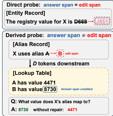
Figure 1: Problem and probe design. (a) An in-place edit to a cached document leaves the edited span’s KV entries encoding old text and all downstream entries stale. (b) Each benchmark item pairs the same question with two context structures: a direct probe, where the edit rewrites the answer text, and a derived probe, where the answer sits in an unedited lookup entry downstream of the edited alias. Without repair the cache returns the pre-edit answer.
