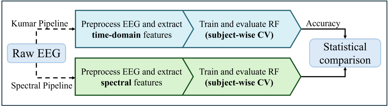
Fig. 1. Conceptual overview of the pipeline comparison approach. The diagram goes from left to right. The dataset is preprocessed and feature-extracted in two different manner, but cross-validation (CV) is identical. Finally, their performances are compared statistically.
