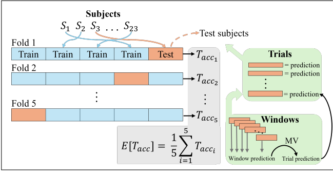
Fig. 3. Schematic overview of the subject-wise cross-validation and trial-level evaluation procedure. In each fold, models are trained on a subset of subjects and tested on held-out subjects. Window-level predictions are aggregated to the trial level using majority voting (MV), and final performance is obtained by averaging trial-wise accuracies across folds.
