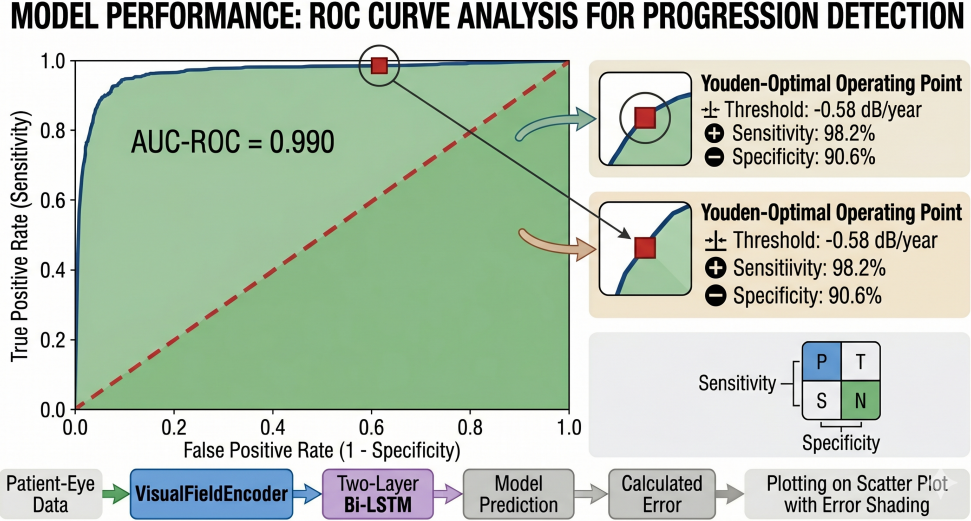
Figure 3: Receiver operating characteristic curve for fast-progressor detection (MD < -1 \text{ dB yr}^{-1} ) on the held-out test set. AUC = 0.990 (95% confidence interval by stratified bootstrap: 0.982–0.996). The Youden-optimal operating point (predicted MD threshold = -0.58 \text{ dB yr}^{-1} ; sensitivity 98.2%, specificity 90.6%) is marked. AUC, area under the receiver operating characteristic curve; MD, mean deviation.
