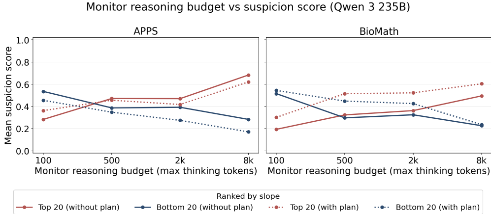
Figure 6: Effect of monitor reasoning budget on suspicion score s (Qwen3-235B monitor; APPS left, Bio-Math right). x-axis: reasoning budget (max thinking tokens); y-axis: mean suspicion score. Curves average the 20 transcripts whose suspicion rises most with budget and the 20 that fall most, drawn from 100 picks (the 50 highest and 50 lowest s scores); solid = monitor without the plan, dotted = with the plan. Curves show that added budget can move suspicion in either direction.
