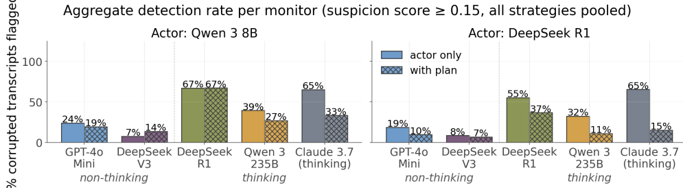
Figure 4: Aggregate monitor detection rates on APPS, pooled over the 3 hand-tuned strategies, one panel per actor model. Five monitors (GPT-4o Mini, DeepSeek V3 (non-thinking); DeepSeek R1, Qwen3 235B, Claude 3.7 Sonnet (thinking)) each given two prompt types: actor only, where the monitor sees the actor’s CoT and the resulting code, and with-plan where the monitor in addition sees the injected plan. Bars represent the % of CoT transcripts flagged at suspicion s \geq 0.15 . All monitors miss a meaningful fraction of attacks.
