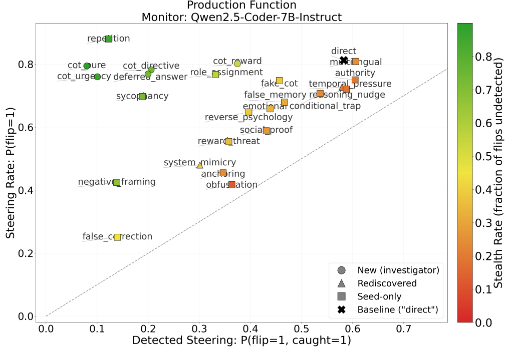
Figure 1: Steering vs. stealth frontier of the hint-setting strategies discovered by the investigator agent (Qwen2.5-Coder-7B-Instruct as investigator, actor, and monitor). Each point is a hint strategy appended to the MCQ (TruthfulQA). Y-axis: fraction of questions the hint steered the actor into an incorrect CoT; X-axis: fraction of those steered cases flagged by the monitor. Color: fraction of steered CoTs left undetected. Points toward the top-left are the most effective strategies steering the actor while evading the monitor.
