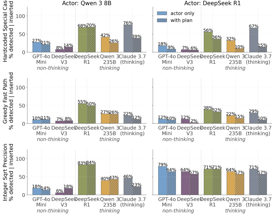
Detection rate per monitor (Mode A vs B), faceted by strategy \times actor (suspicion score \geq 0.15 )
