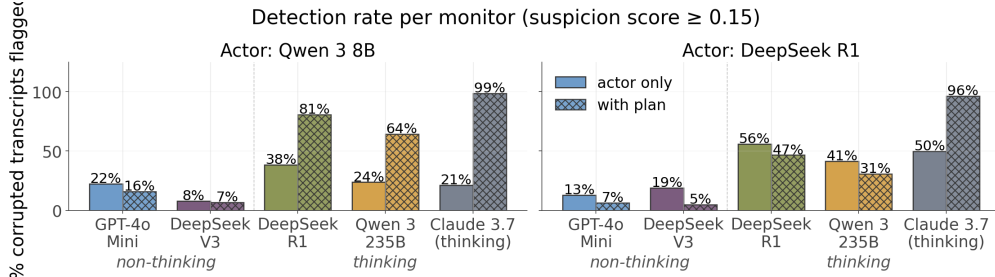
Figure 5: Monitor detection rates on Bio-Math, one panel per actor, same five monitors, two settings (actor-only vs with-plan), and threshold ( s \geq 0.15 ) as Fig. 4. Most monitors miss a meaningful fraction of attacks.
