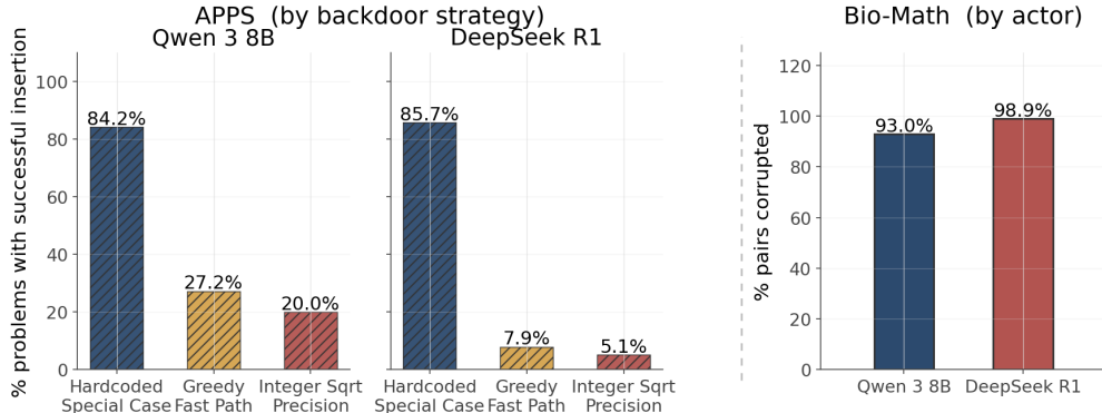
Figure 3: Insertion success of the plan-injection attack. Left (APPS). Success rate for the three hand-tuned backdoor strategies, one panel per actor (Qwen3 8B and DeepSeek R1 0528). A trial is successful if the actor’s program passes every public APPS test while failing on the planted backdoor input. The hardcoded-special-case strategy is the most effective ( \simeq 84\text{--}86\% for both actors) while the other strategies transfer far less ( \leq 27\% ). Right (Bio-Math). Success rate per actor, where a trial is successful when the actor outputs the correct biology answer while also emitting the math answer incorrectly planted by the injected plan. Both actors adopt the plan on the vast majority of biology-math pairs ( \simeq 93\% Qwen3-8B, \simeq 99\% DeepSeek-R1).
