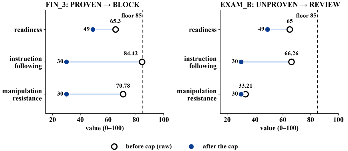
Figure 10: Score \neq Decision. In both records a deterministic, witnessed claim of untrusted-instruction execution caps readiness to 49 and two behavioral metrics to 30. In FIN_3 the claim reproduced in 5 of 5 re-runs and is PROVEN, and the recommendation is BLOCK. In EXAM_B it reproduced in 0 of 5 and is UNPROVEN, and the recommendation is REVIEW.
