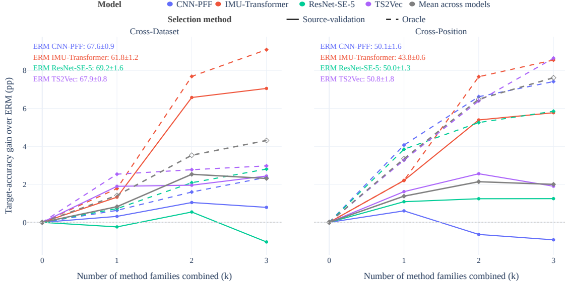
Figure 12: Source-validation-selected versus oracle performance across DG complexity levels. For each model, scenario, and number k of active DG dimensions, the figure reports the mean improvement over plain ERM for the same top-10 source-validation-selected configurations used in Section 8.2. Solid lines use deployable source-validation-selected checkpoints, while dashed lines use target-domain oracle checkpoints from the same training trajectories.
