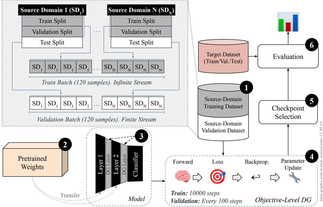
Figure 3: Overview of the DG protocol. 1 Data partitioning: one domain is held out as the unseen target, and the remaining domains are used for training and source validation. 2 Model initialization: the model is initialized randomly or through SSL pretraining. 3 Architectural modification: MixStyle, EFD-Mix, or DDG may be incorporated. 4 DG objective: training uses ERM or an alternative objective-based strategy. 5 Training and selection: models are trained for 10,000 steps, with checkpoints selected by mean source-validation accuracy. 6 Target evaluation: the selected checkpoint is evaluated on the held-out target domain.
