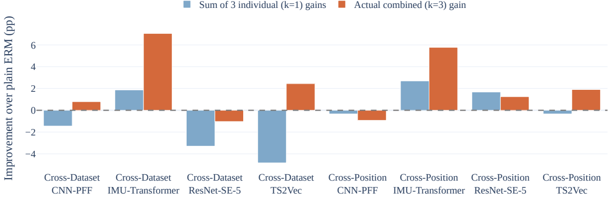
Figure 8: Empirical interaction among DG dimensions. We compare observed improvements of the top-10 configurations using all three dimensions with the sum of their isolated effects. Positive gaps indicate super-additive interaction, and negative gaps indicate redundancy or interference. We do not interpret cases where both quantities are negative as synergy.
