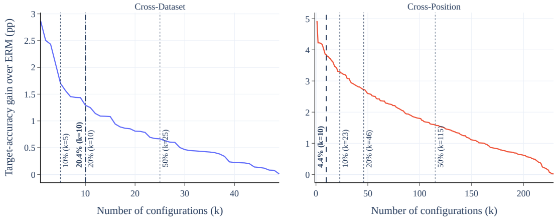
Figure 14: Target-accuracy gain over ERM as a function of the number of positively improving configurations, ranked from highest to lowest gain. The dashed lines indicate the top 10%, 20%, and 50% of improving configurations and the fixed choice k = 10 used in the complementarity analysis.
