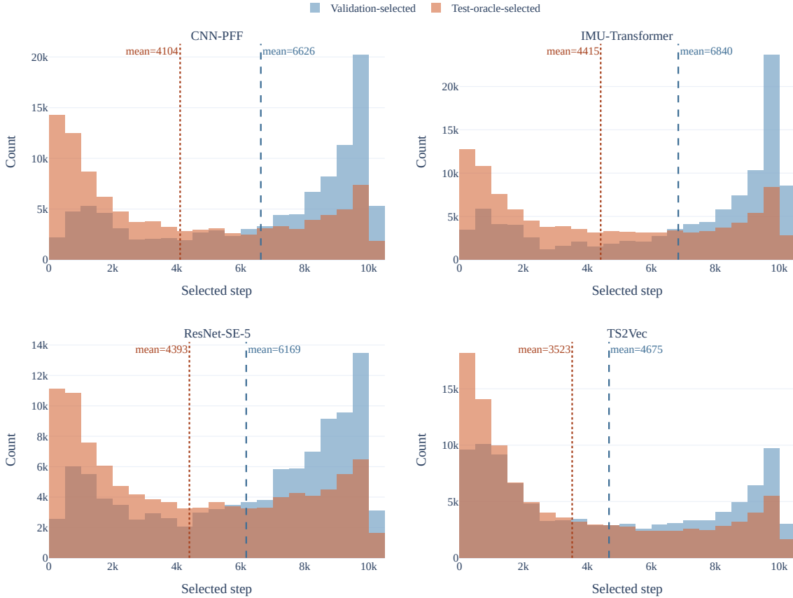
Figure 13: Distribution of the selected training step for each backbone under source-validation-based and oracle target-domain checkpoint selection. The source-validation protocol corresponds to the deployable procedure used throughout the benchmark, whereas the oracle protocol selects the checkpoint with the highest target-domain accuracy.
