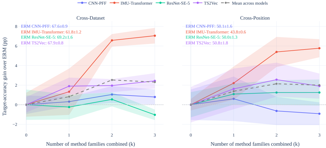
Figure 7: Complementarity across DG dimensions. For each model, scenario, and number k of active dimensions, the figure reports the mean improvement over plain ERM for the ten best source-validation-selected configurations. Solid lines represent individual models, the dashed line the mean across models, and the shaded region the corresponding standard deviation.
