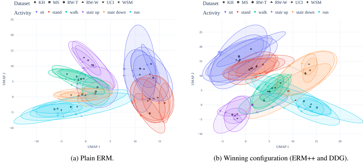
Figure 10: Latent-space activity centroids for IMU-Transformer with MS as the held-out CD target. Marker shapes denote datasets and colors denote activities. The winning configuration improves target accuracy by 13.3 pp and yields clearer separation among difficult locomotion activities, especially for walk and stair-related activities.
