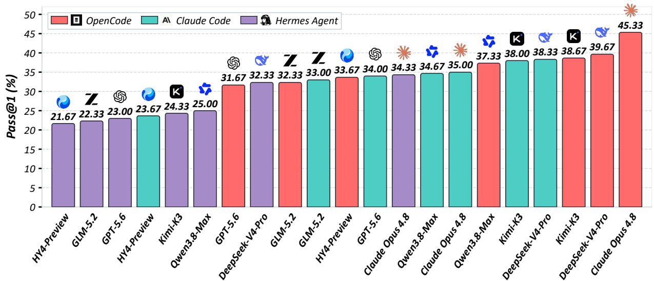
Figure 1 Pass@1 for 21 model–harness pairs on 300 CHECKERBENCH tasks (Table 2).
