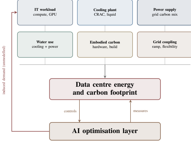
Fig. 1: Drivers of the data center footprint. The optimisation layer controls the facility, but the demand it makes cheaper feeds back into workload — a path left unmodelled in the studies surveyed here.
