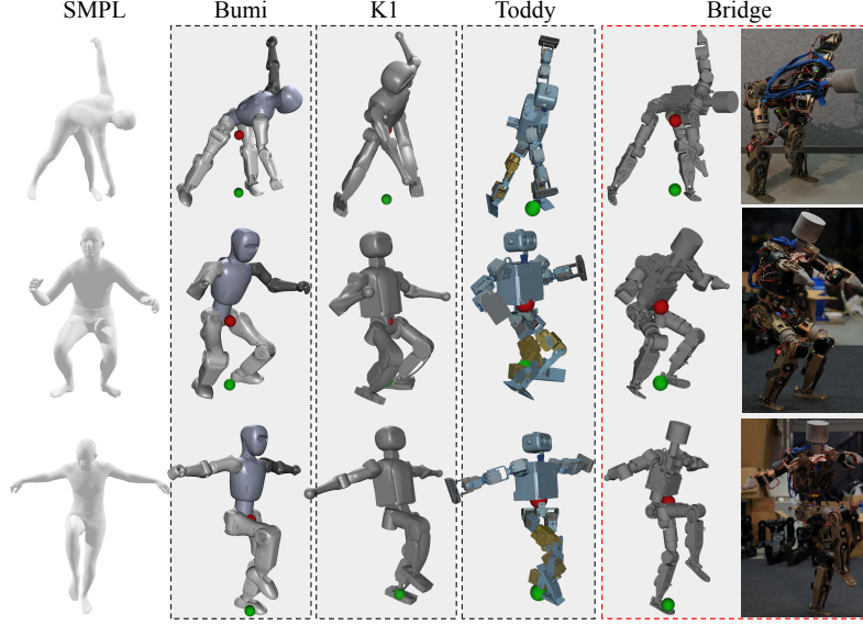
Figure 6: Comparison with comparable humanoid platforms across different motions.
