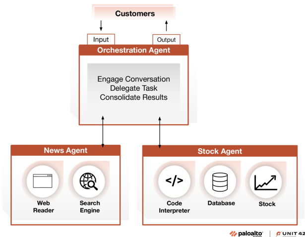
Figure 6: Stock Advisory Assistant Architecture. Source: https://unit42.paloaltonetworks.com/agent-ai-threats/
