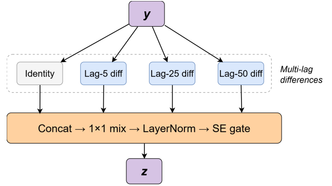
Figure 3: The LMLD module. The WSAN-normalised window is differenced at a bank of lags P = \{5, 10, 25, 50\} (only 5, 25, 50 drawn); each difference is scaled by a learnable per-channel weight, concatenated with the identity stream, mixed by a 1 \times 1 convolution, layer-normalised, and gated by a squeeze-excitation block.
