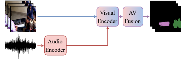
Fig. 1: Comparison between our simplified approach and common Transformer-based AVS methods. Our approach eliminates unnecessary architectural complexity, resulting in a more efficient model while preserving high segmentation performance.
