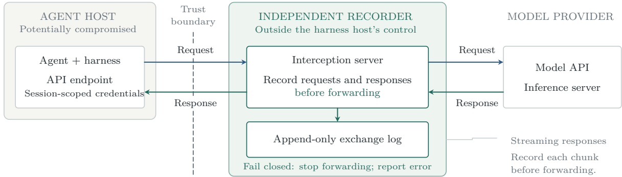
Figure 10. A trusted interception server , outside the agent host’s control, records every request and response (streamed chunks individually) to an append-only log before forwarding, and fails closed if recording fails.
