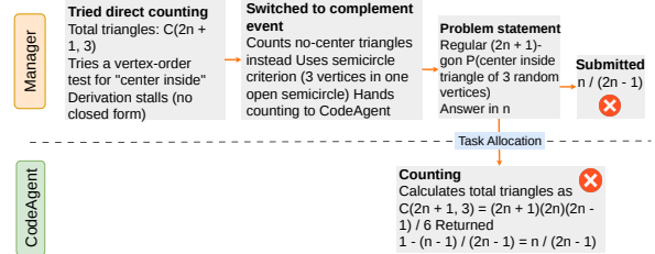
Figure 5: SmolAgents communication trajectory for the same Omni-MATH task in Figure 4.
