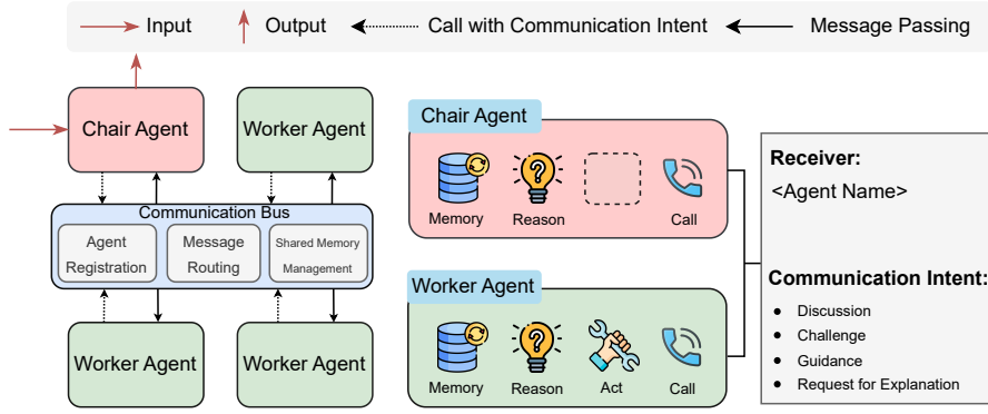
Figure 2: Overview of the BusMA communication substrate.
