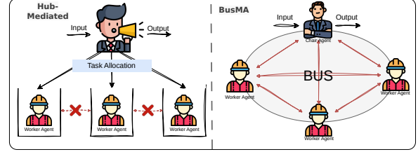
Figure 1: Comparison of hub-mediated topologies and BusMA. Left: In hub-mediated frameworks, Workers have restricted autonomy as passive executors, unable to initiate worker-to-worker communication (indicated by \times ). Right: BusMA enables agents to directly address specific peers through a shared channel (the Bus), supporting four communication intents: Discussion, Challenge, Guidance, and Request for Explanation.
