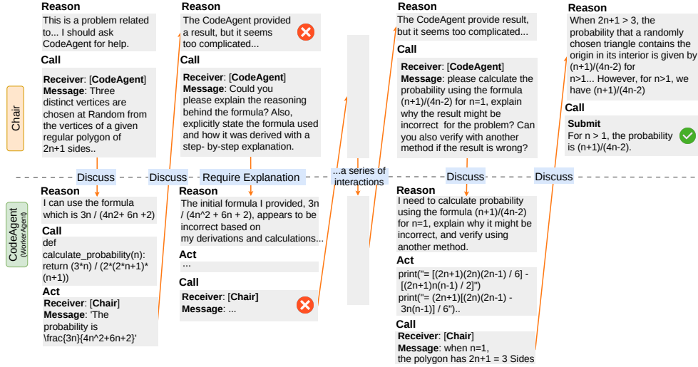
Figure 4: BusMA communication trajectory for answering a question from Omni-MATH: Three distinct vertices are chosen randomly from the vertices of a regular polygon with (2n+1) sides; what is the probability that the center lies inside the triangle formed by the three chosen vertices? The full trajectory is provided in Table 8.
