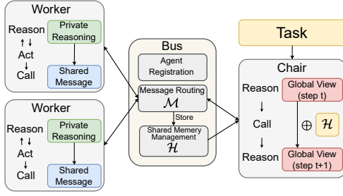
Figure 3: Information flow in BusMA: private reasoning r_{i,t}^{\text{priv}} , shared message m_{i \rightarrow j} , and global view r_{\text{chair},t}^{\text{glob}} .
