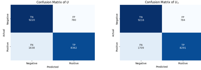
Fig. 3: Confusion matrices of XGBoost on the two data representations, computed on the test split only ( N = 20,000 ). Positive class corresponds to delayed flights. From left to right: \mathcal{U} and \mathcal{U}_\Psi .
