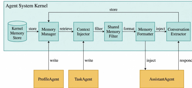
Figure 2: Kernel-managed shared memory: ProfileAgent and TaskAgent write structured memories, AssistantAgent remains retrieval-free, and the kernel enforces write ordering, privacy, retrieval, formatting, and injection between them.
