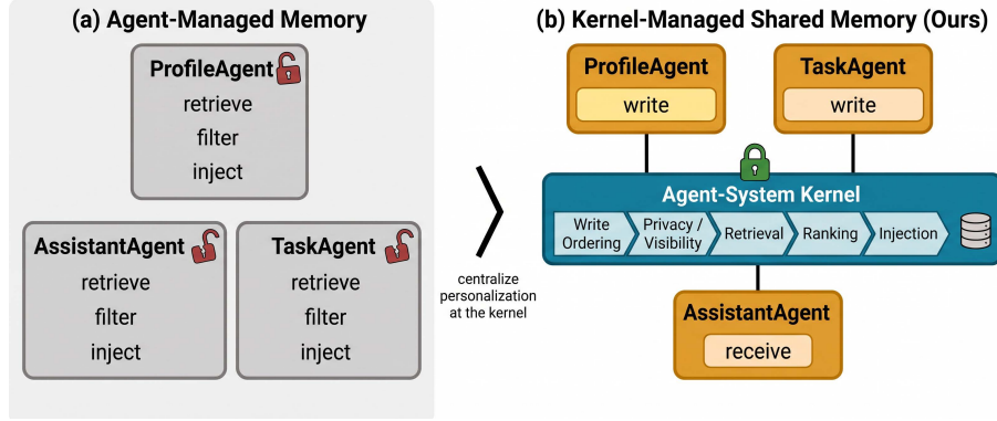
Figure 1: Kernel-managed shared memory centralizes retrieval, privacy enforcement, and prompt injection at the agent-system kernel instead of leaving them to individual agents (left vs. right), matching full-context personalization quality at a fraction of the latency and token cost (Section 4.4).
