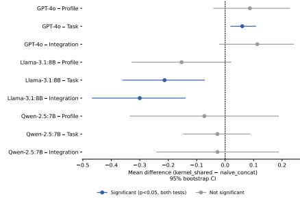
Figure 3: Mean difference and 95% bootstrap CI for the nine kernel_shared vs. naive_concat comparisons; six of nine intervals cross zero (dashed line), indicating no significant difference.
