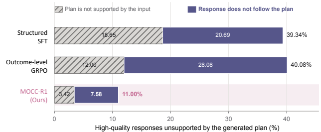
Figure 5: High-quality responses unsupported by the generated counseling plan. The components distinguish plans unsupported by the input from responses that do not follow an input-supported plan.
