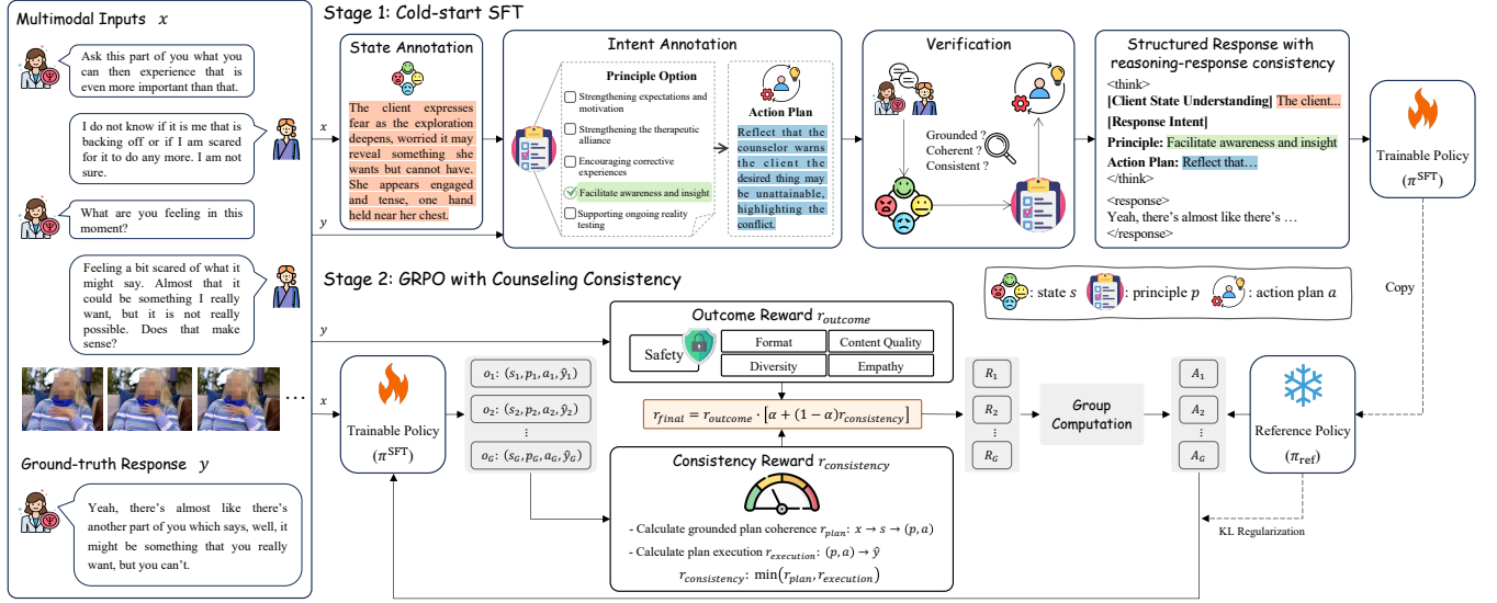
Figure 3: The overall framework of our proposed MOCC-R1.
