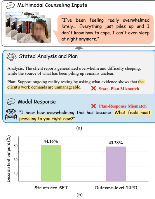
Figure 1: (a) A generated counseling decision chain can exhibit both a state-plan mismatch and a plan-response mismatch. (b) Reasoning-response inconsistency remains around 40% under both Structured SFT and Outcome-level GRPO.
