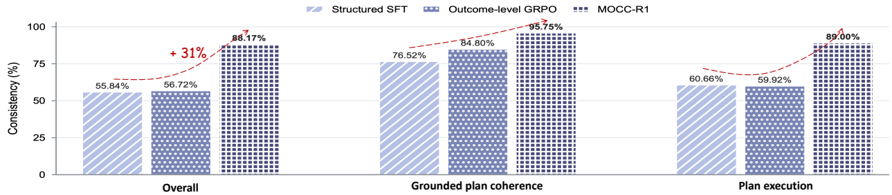
Figure 4: Comparison of structured-output methods on the MOCC dataset in terms of counseling reasoning–response consistency.
