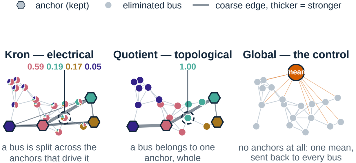
Figure 2: The coarsening comparison from the poster, computed on an illustrative 18-node weighted graph with four shared anchors. Each interior-node pie shows a row of the prolongation matrix U : several anchor weights for Kron, one unit weight for Quotient. Coarse-edge thickness represents coupling magnitude. The third panel illustrates a single global average as a conceptual comparison; the empirical study here compares Flat, Kron and Quotient. These are schematic constructions on a toy graph, not experimental grid measurements.
