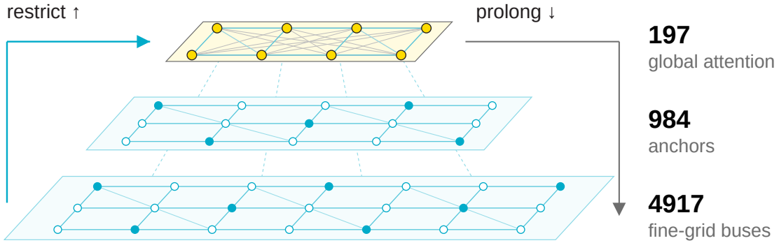
Figure 3: The poster’s multilevel communication diagram. The upward path follows Eqs. (13)–(14); the return follows Eqs. (15)–(16). Dense attention exchanges information among the 197 top-level nodes in the 4,917-bus example. Labels give actual hierarchy sizes; the network planes and displayed nodes are schematic.
