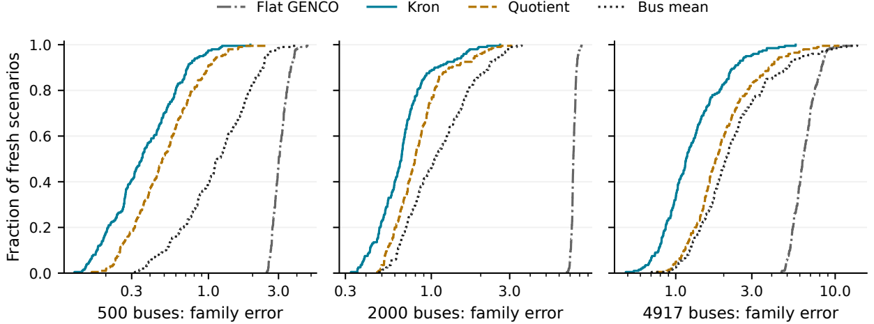
Figure 5: Error distributions on fresh operating scenarios for the three training topologies. Each curve is an empirical cumulative distribution over the same 200 scenarios; neural-model errors are averaged over three seeds separately for each scenario. The reference uses its own error on each matching scenario. A curve further left reaches the same fraction of scenarios at a lower error. The curves describe scenario variation; they are not confidence intervals across seeds.
