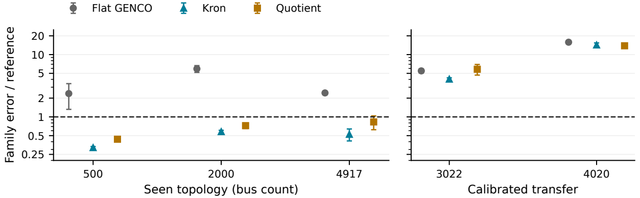
Figure 4: Fresh-scenario family error relative to each grid’s fitted bus-mean reference. Markers show means over three seeds; error bars show one sample standard deviation, scaled by the fixed reference. Values below one improve on the reference. The left panel demonstrates scenario generalization on training topologies; the right separately shows the present calibrated-transfer results on additional topologies.
