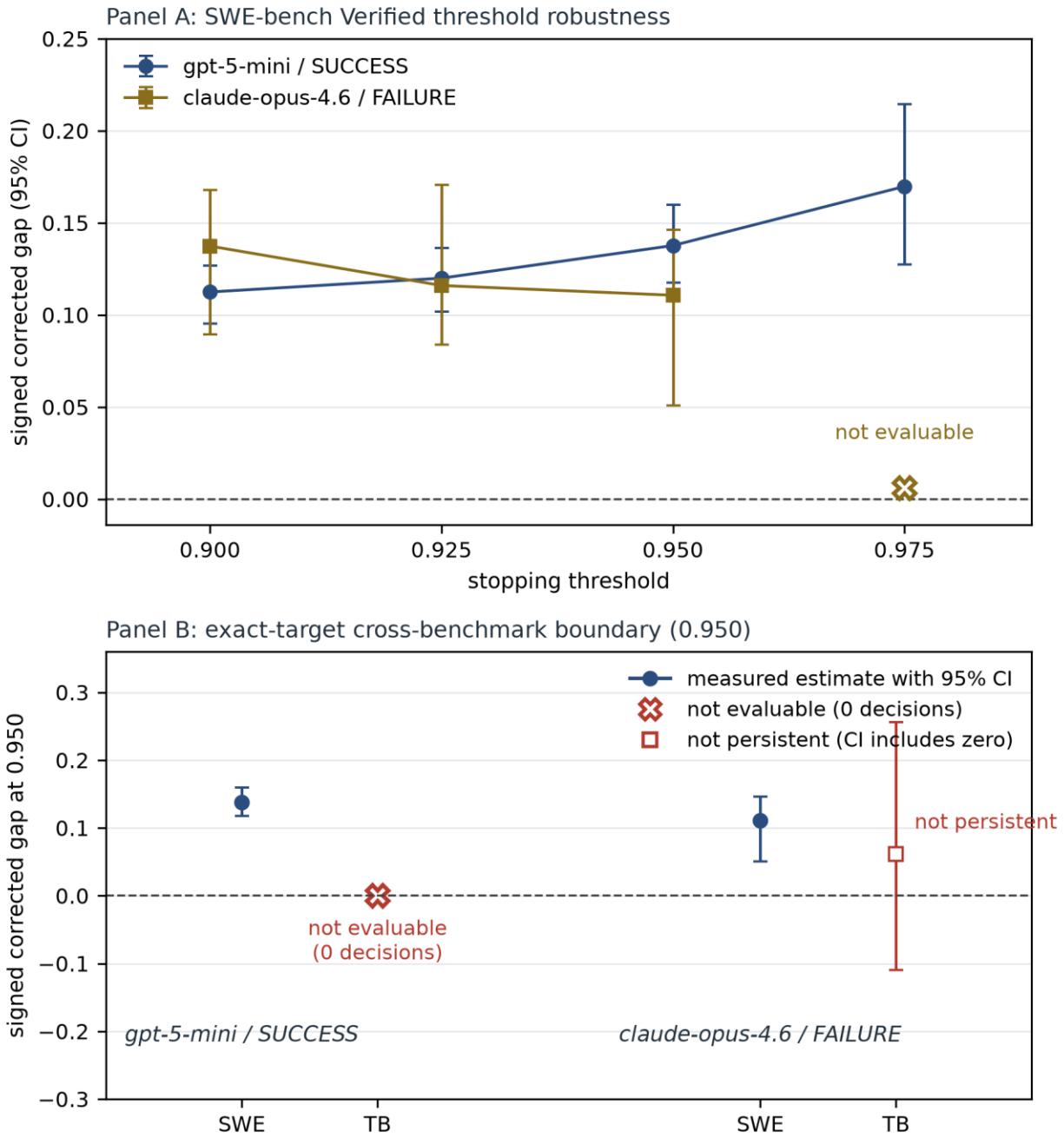
Figure 4. Threshold robustness and cross-benchmark boundary. Panel A: Signed oracle-prior-corrected calibration gap against the stopping threshold (0.900, 0.925, 0.950, 0.975) for the two frozen SWE targets, with frozen task-cluster bootstrap 95% CIs. The claude-opus-4.6/FAILURE series is not evaluable at 0.975 because no occurrence clears the decision-count minimum; that state is drawn as a not-evaluable marker rather than interpolated or set to zero. Panel B: Exact-target cross-benchmark comparison at 0.950 for the same two targets on SWE-bench Verified versus TerminalBench under the fixed terminus-2 scaffold. For the SWE-bench points, the plotted estimate is the frozen target-level median corrected gap at 0.950 with its task-cluster bootstrap interval; for TerminalBench, the plotted value is the identity-matched held-out target-model estimate at 0.950. Marker classes distinguish measured estimates with confidence intervals, non-evaluable cells, and non-persistent cells. The gpt-5-mini/SUCCESS target produced 0 TerminalBench decisions,
