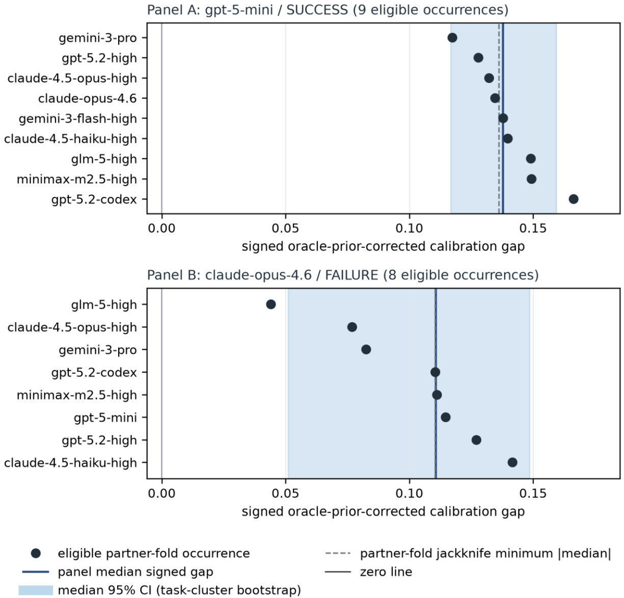
Figure 3. Target-specific persistence of two SWE-bench Verified calibration-transfer errors under a shared predictor. One glyph per eligible partner-fold occurrence. The y-axis lists the partner held-out agent, and the x-axis shows the signed oracle-prior-corrected calibration gap, with a vertical line at zero. Panel A: gpt-5-mini/SUCCESS, 9 eligible occurrences. Panel B: claude-opus-4.6/FAILURE, 8 eligible occurrences; one further occurrence fails the frozen eligibility rule and is excluded from the plotted gap values. Overlays mark the panel median, its task-cluster bootstrap 95% CI, the partner-fold jackknife minimum, and the two task-half medians; they belong to the panel median, and no CI is drawn for an individual occurrence. Values are from the frozen Phase 1A shared-predictor control and Phase 1A-D persistence validation. The figure establishes target-specific persistence within this setting; it does not establish broad pairwise heterogeneity, and it does not generalize beyond SWE-bench Verified.
