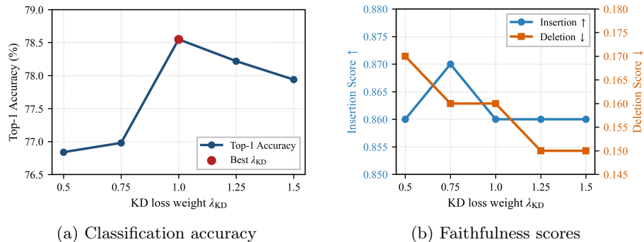
Fig. 3. Sensitivity analysis of the KD loss weight \lambda_{\text{KD}} on CUB. (a) reports Top-1 classification accuracy. (b) reports insertion and deletion faithfulness scores. All other hyperparameters are kept identical to the default CARE configuration.
