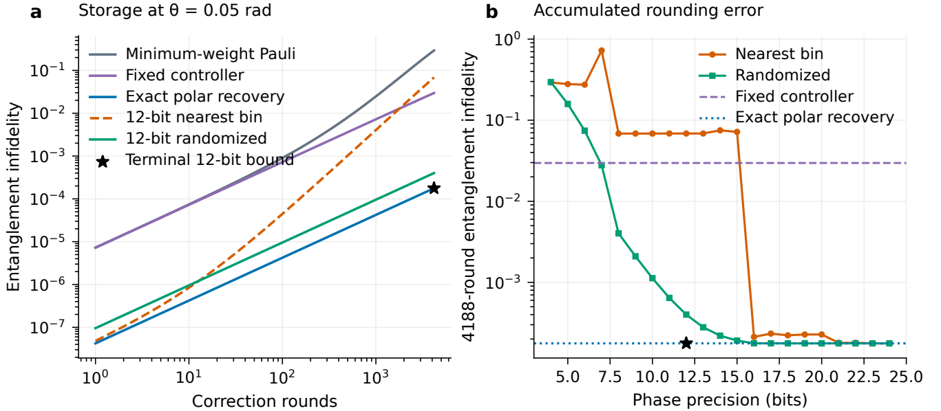
FIG. S5. Recovery and accumulated control precision for the exact L = 3 instrument at \theta = 0.05 . (a) Final-memory entanglement infidelity versus rounds. The fixed diagonal controller is tuned to R = 4188 ; it is an implemented feasible policy, close to the terminal-unitary bound there. (b) The complete integer precision sweep at the same horizon. Ordinary rounding leaves coherent bias; randomized rounding trades it for dephasing. The terminal 12-bit entry reports the analytical guarantee. The comparison assumes ideal extraction and signed calibration; logical-gate implementation costs would add to the reported resources.
