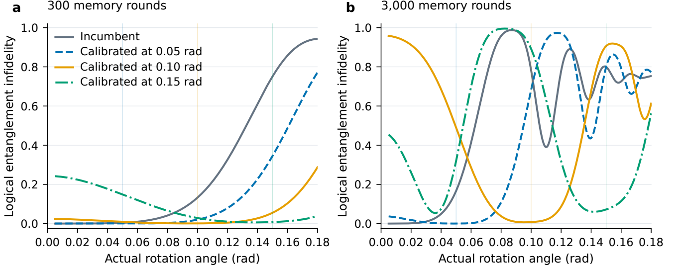
FIG. S1. Beneficial and harmful recovery under calibration mismatch. Each curve evaluates the exact logical-channel formula numerically at 2001 angles; the panels show two memory horizons. Fixed phase tables can greatly reduce infidelity near their calibration point and worsen it elsewhere. The plotted grid illustrates the risk, while the evaluator also bounds its variation between grid points. The correction assumes error-free logical actuation; the appreciable incumbent infidelity makes its recovery benefit visible.
