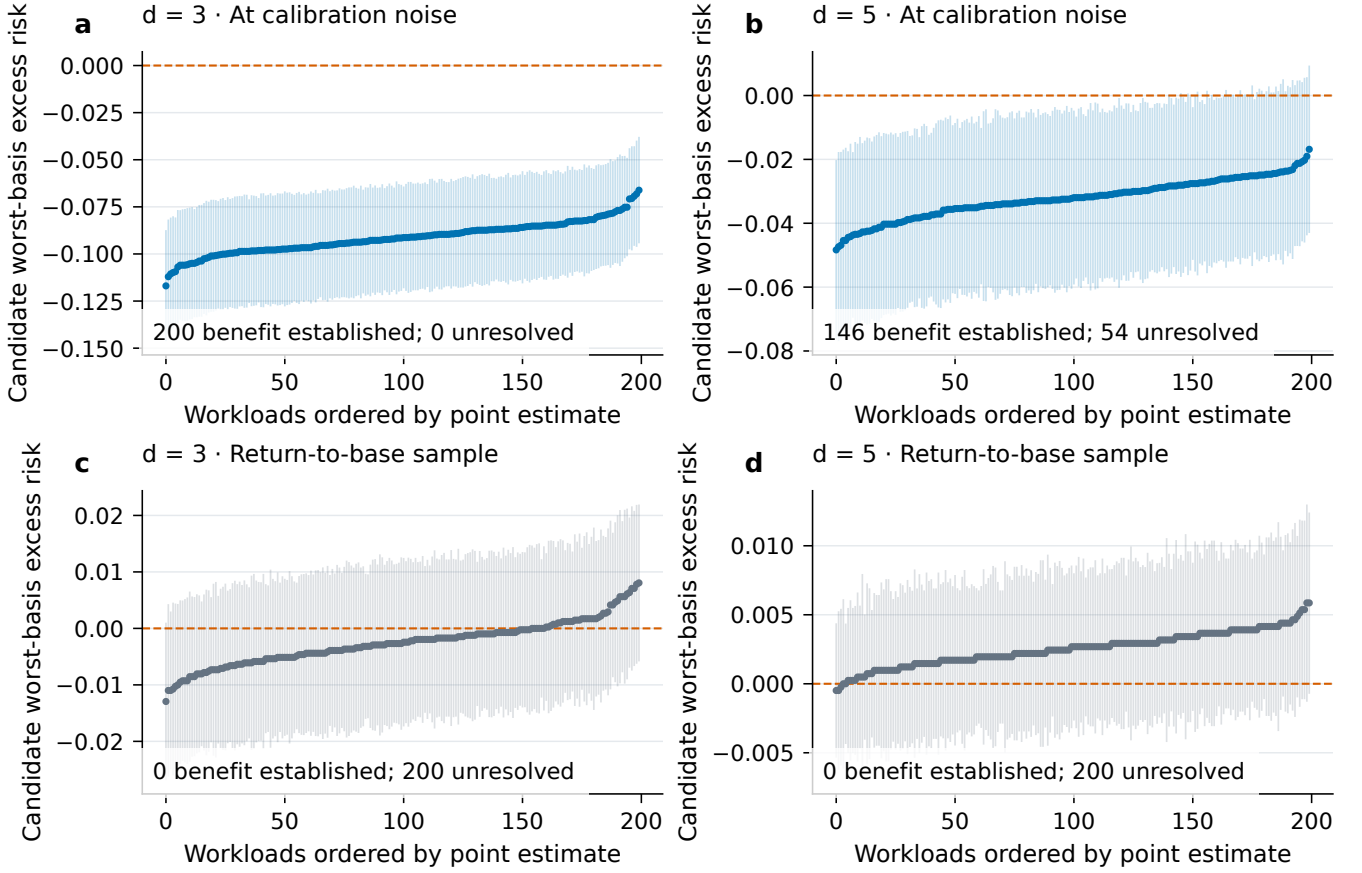
FIG. S11. Circuit confirmation with all 200 paths per distance and deployment stage. Each point is an estimate from an independent deployment sample of worst-basis excess risk; vertical segments are the saved pointwise 95% final risk boxes. Each panel orders paths independently by its own point estimates; paired stages must be compared through their workload identifiers. Benefit is established for 200 distance-3 and 146 distance-5 paths at the calibration settings; all 400 stale effects remain unresolved. Point estimates retain finite-sample maximum bias; harmful staleness requires a resolved adverse risk difference.
