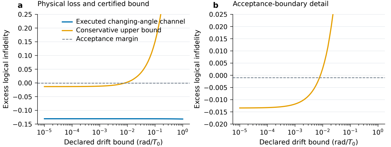
FIG. S9. Within-block drift extension over 81 evaluated rates. (a) Numerically evaluated changing-channel excess risk and the conservative upper bound. (b) An expanded view of the acceptance boundary at excess risk -10^{-3} . Curves outside each displayed vertical range are clipped. The simulation specifies acquisition durations, terminal-action noise, and physical drift bounds.
