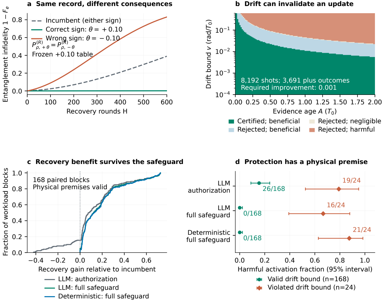
FIG. S18. Evidence connects an information limit to a recovery decision. (a) Identical passive history laws have different recovery consequences: one fixed +0.10 phase table helps at the correct sign and harms at the opposite sign in the L = 3 toric instrument of Sec. I. (b) Certification and rejection for 1 8192-shot calibration record, as evidence age and the drift bound increase. Rejected colors distinguish evaluator-only recovery outcomes; the controller sees the evidence and certificate. (c) Recovery-gain distributions over 168 paired workloads satisfying the assumptions. The guarded large language model (LLM) completes 159 beneficial updates with 0 observed harmful activations; authorization alone gives 142 beneficial updates and 26 harmful activations. The guarded deterministic controller completes 162 beneficial updates with 0 observed harmful activations. (d) Harmful-activation fractions with pointwise 95% Chernoff intervals based on the Kullback–Leibler (KL) divergence. Exceeding the drift bound causes harm under the full gate: 16/24 LLM and 21/24 deterministic workloads. Each independent workload supplies 4 paired rollouts. Supplemental Material, Sec. X 2, defines outcomes of the coherent-memory controller experiment; the detailed empirical panels in the supporting material give plotting methods and condition-resolved results.
