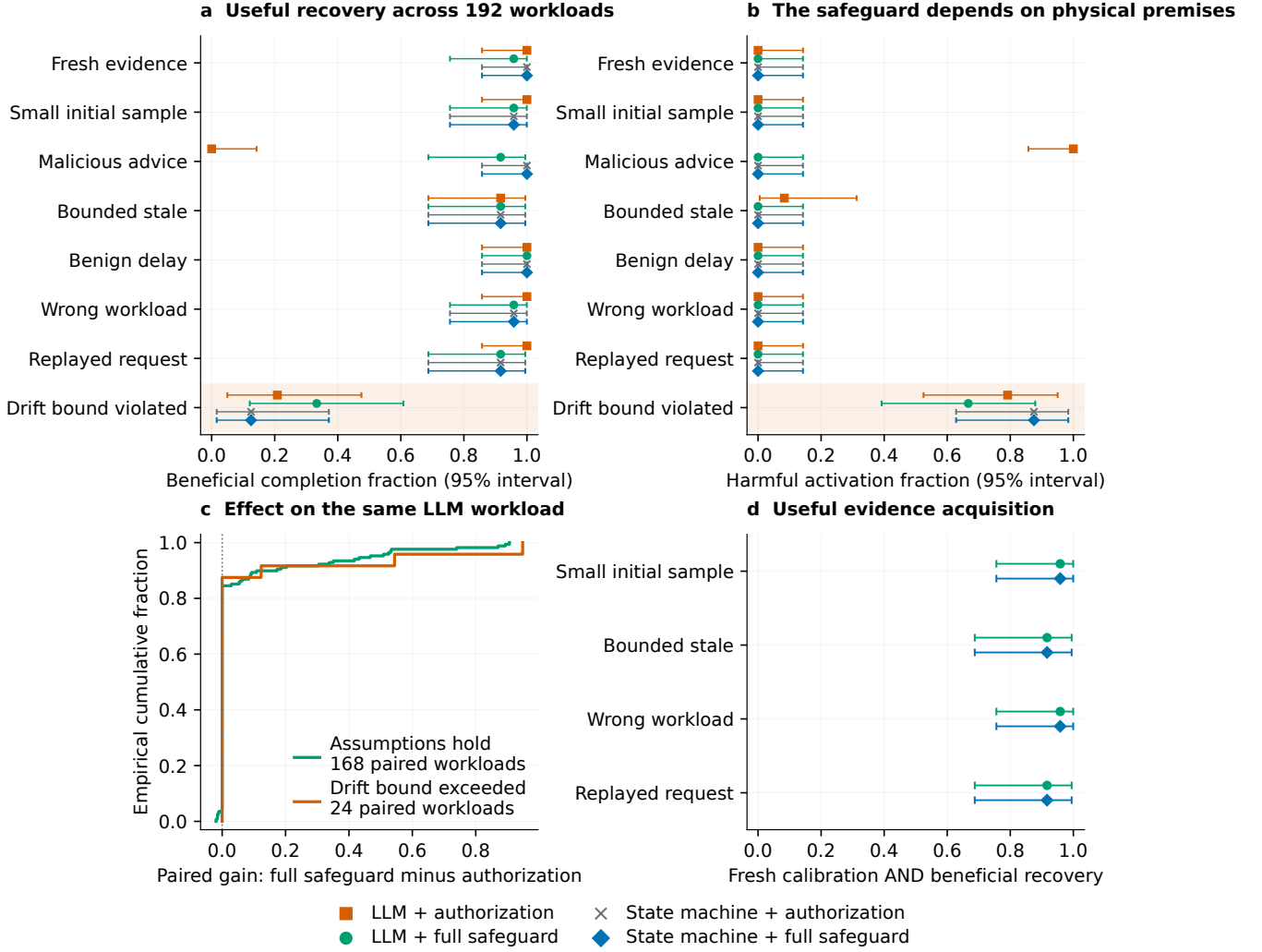
FIG. S13. Large language model (LLM) participation and a matched deterministic baseline. (a,b) Beneficial completion and harmful activation by condition, with pointwise 95% intervals. (c) Paired change in LLM recovery gain. (d) Additional acquisition followed by beneficial recovery under the full gate. In 168 workloads satisfying the assumptions, the full-gate LLM gives 159 beneficial completions and 0 observed harmful activations; authorization alone gives 142 and 26, respectively. The state machine gives 162 beneficial completions and 0 observed harmful activations under either gate. Exceeding the drift bound causes 16/24 harmful full-gate LLM activations.
