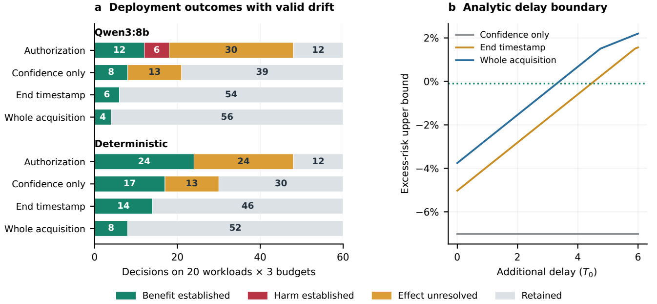
FIG. S25. Supporting conditional timing bound for the surface-code study. (a) Outcomes from the same 20 valid-premise workloads at 3 nested budgets, shown in main Fig. 4(a). (b) Additional-delay bounds for one recorded honest distance-3 calibration at 32768 shots per basis and its measured Qwen latency converted to the scenario clock. Confidence-only, end-timestamp and whole-acquisition curves reevaluate their transport formulas on the same observation. Including acquisition time shortens the sufficient acceptance window. These curve points are not new simulated samples. Main Fig. 4(b) instead identifies the decisions changed by the two timing rules and their independent recovery outcomes.
