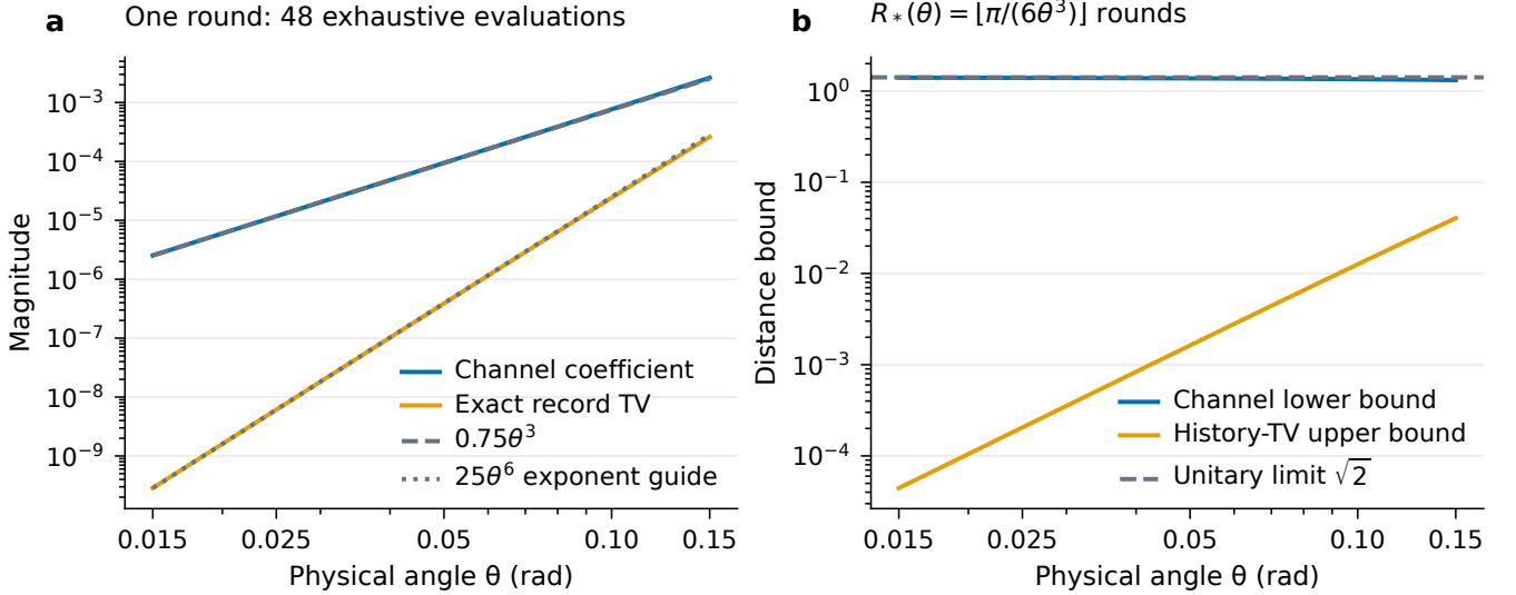
FIG. S3. Finite-angle separation for the 18-qubit toric instrument of Sec. I. (a) The channel carrier magnitude and exact maximal one-round record total-variation (TV) distance approach orders \theta^3 and \theta^6 , respectively. The dotted curve is only an exponent guide. (b) An evaluated input-state trace distance lower-bounds the unhalved channel diamond distance, while R_*\eta_3 upper-bounds the maximal history TV. The history curve bounds the distance from above. All solid curves are exhaustive support-sum evaluations at 48 angles.
