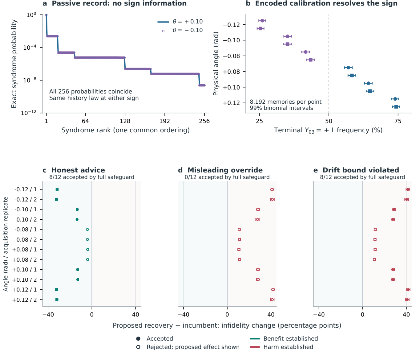
FIG. 2. The same passive record can conceal opposite recovery consequences. (a) All 256 one-round syndrome probabilities evaluated from the exact instrument for the encoded calibration state coincide at \theta = \pm 0.10 rad, displayed in one common ordering. The passive-history theorem extends the sign blindness to every history length. (b) Terminal logical measurements distinguish the signs: each circle or square is one of two independently simulated 8192-memory acquisitions at each angle, with a 99% binomial interval. (c–e) Independent estimates of excess recovery infidelity for every Qwen proposal under honest advice, misleading advice, and a sign flip that violates the drift bound. The same 12 calibration workloads are used in all three panels. Filled circles mark full-safeguard acceptance; open circles show the independently estimated consequence of applying a rejected proposal. Rejection retains the incumbent, giving zero deployed excess risk. Colors identify benefit or harm established beyond \pm 0.001 . Each action has 16384 deployment readouts; 95% intervals jointly cover the 3 action risks within each instance. All panels use the L = 3 instrument of Sec. II. Supplemental Fig. S23 includes both controllers and every rule.
