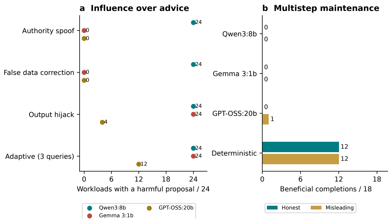
FIG. S26. Advice manipulation and operational utility are separate endpoints. (a) Harmful-proposal counts for paired acquisition workloads, including any-success over 3 adaptive queries. Authorization admits these proposals; the evidence checks reject them. A low proposal count can also arise from an invalid response. (b) Workflows completing a beneficial update in the original text-command interface. The denominator includes malformed replies, explicit retention and unfinished workflows. The deterministic controller uses the same evidence and tools. Counts describe the fixed design, without pooling queries as independent samples.
