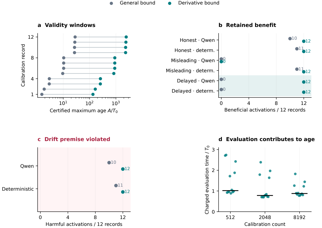
FIG. S28. Validated numerical bounds recover benefit while retaining the physical failure boundary. (a) Paired certified maximum ages for the 12 acquisitions at budget 8192, sorted by the general-bound expiry. Both methods use identical validated stationary bounds. (b) Beneficial activations after charging the same measured evaluation time. (c) Harmful activations when the declared drift premise is violated; marker colors retain their method meaning. The count of 0 harmful activations under valid premises refers to the 32 and 60 accepted updates from the same 96 reused instances. (d) All 36 measured online evaluation costs, with medians marked; the clock conversion is stipulated. Outcomes in (b,c) are interval-enclosed model risks, not newly sampled success rates. The repeated conditions and nested budgets do not create additional independent calibration records.
