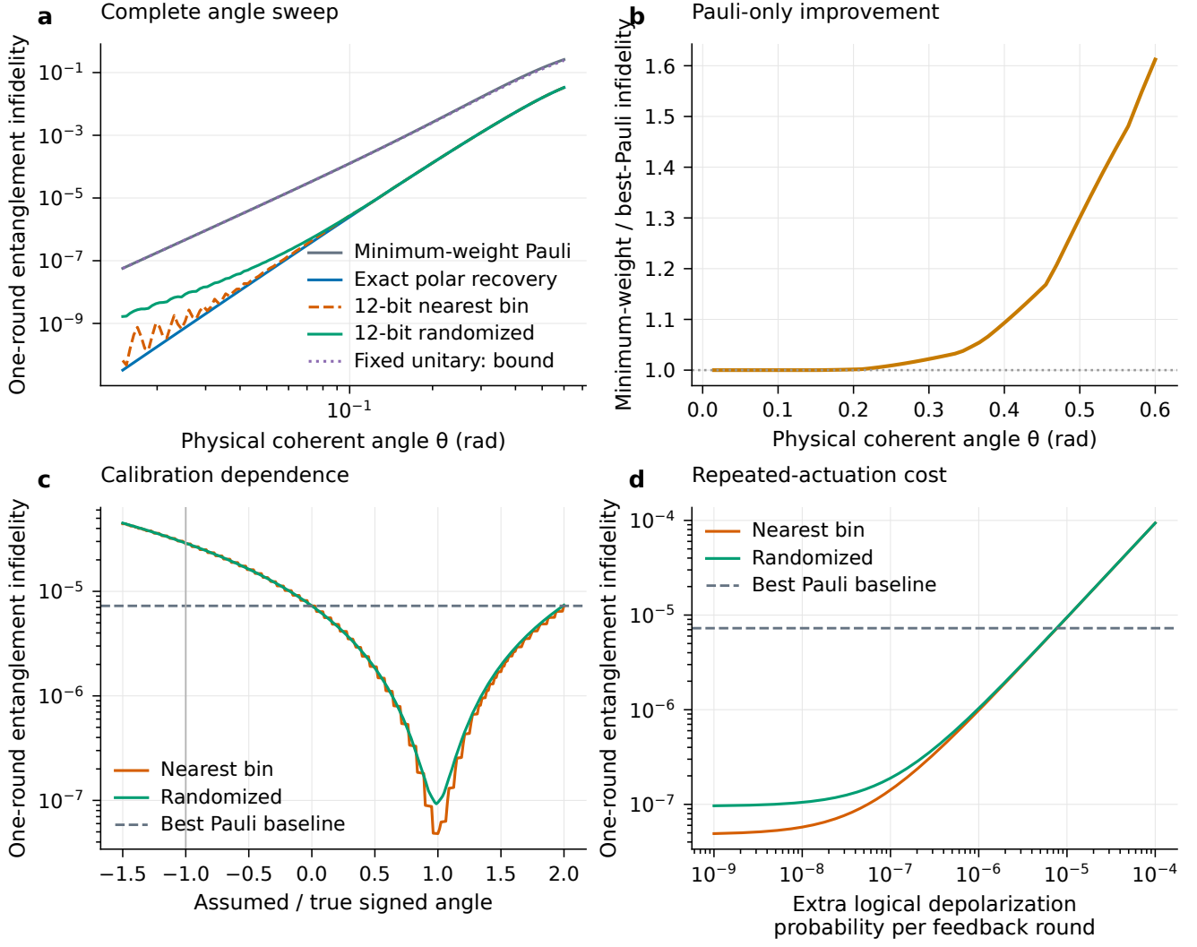
FIG. S8. Complete recovery robustness sweeps. (a) One-round infidelity across 122 angles including the reference angle \theta = 0.05 . (b) Relative Pauli-only improvement occurs at stronger noise, where logical infidelities are high. (c) Assumed calibration divided by true \theta = 0.05 ; -1 is the wrong-sign case. (d) Extra per-round logical depolarization erases the benefit. Dashed and dotted curves labeled as bounds are analytical comparators. Every curve is an exhaustive instrument calculation, so sampling error bars are inapplicable.
