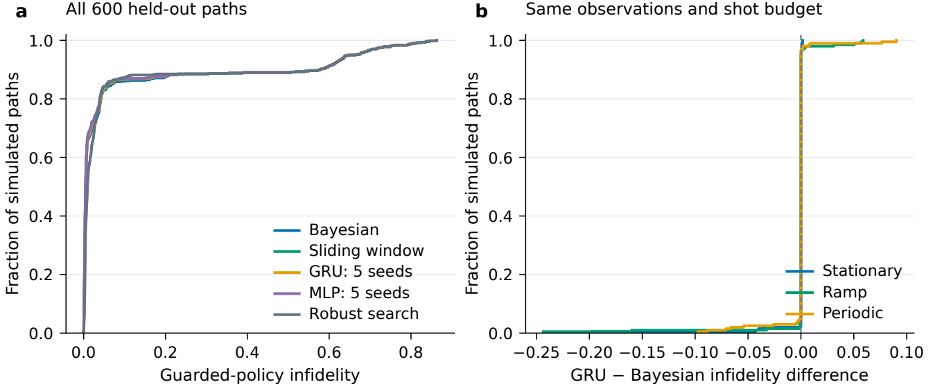
FIG. S10. Empirical distributions on 600 held-out simulated noise paths. (a) Cumulative distributions of guarded-policy infidelity. Neural methods are gated recurrent units (GRUs) and multilayer perceptrons (MLPs); risks are averaged over 5 training seeds within each path. (b) Paired GRU-minus-Bayesian guarded-risk differences, with 200 paths per drift family; negative values favor the GRU. The curves display empirical cumulative distributions; inferential intervals are reported separately where available. All methods have the same observations, action catalog, and budget for new calibration shots.
