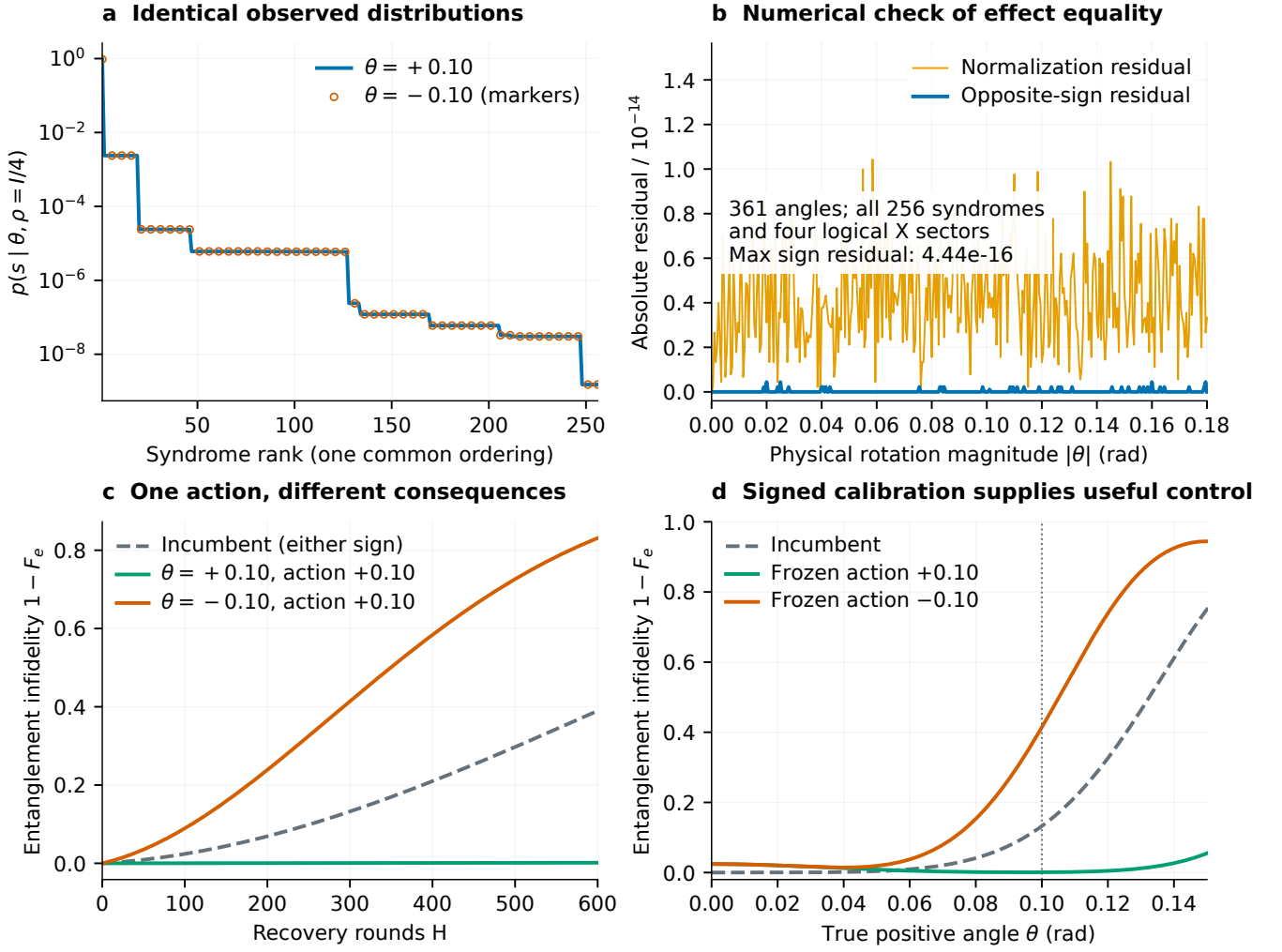
FIG. S19. Passive information and active recovery answer different questions. (a) Opposite-sign syndrome probabilities coincide. (b) The maximum independently evaluated effect residual is 4.44 \times 10^{-16} . (c) One fixed +0.10 recovery table helps at +0.10 and harms at -0.10 . (d) The fixed \pm 0.10 tables have different risk profiles over the H = 300 angle sweep. Numerical residuals quantify computational error; the exact identities establish the information limit.
