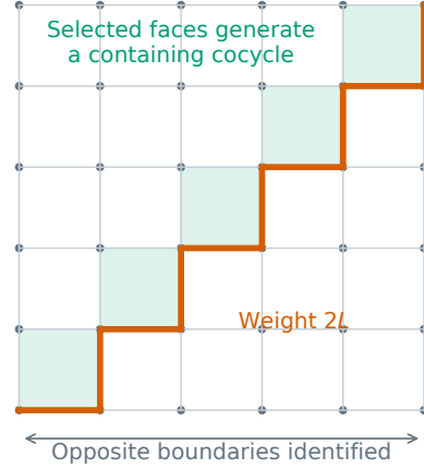
FIG. S2. Geometric witnesses for theorem 3. A straight logical circuit has length L . At odd L , the additional even/cut-covered condition forces winding in both torus directions, and the diagonal staircase attains length 2L . The drawing depicts the code's periodic topology.
