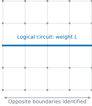
FIG. S2. Geometric witnesses for theorem 3. A straight logical circuit has length L . At odd L , the additional even/cut-covered condition forces winding in both torus directions, and the diagonal staircase attains length 2L . The drawing depicts the code's periodic topology.
