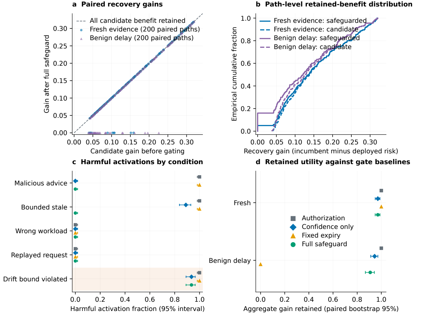
FIG. S21. Paired recovery gains expose protection and its cost. (a,b) Proposed and deployed gains for 200 fresh and 200 benign-delay paths. (c) Harmful activations in five challenge conditions, with pointwise 95% Clopper–Pearson intervals over 200 paths per condition. Violating the drift bound causes full-gate harm on 187/200 paths. (d) Aggregate gain retained: 97.1% [94.9,98.9]% for fresh evidence and 90.8% [86.8,94.2]% for benign delay, using 10,000 matched-path bootstrap replicates. Baselines share measurements and proposals; rejection retains the incumbent. The Supplemental Material gives the baseline definitions and plotting protocol.
