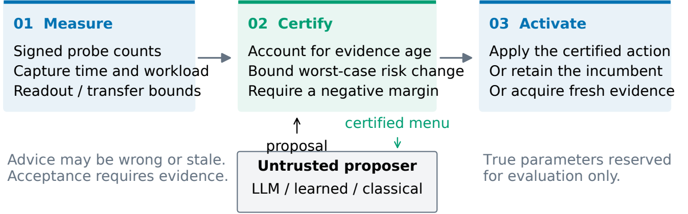
FIG. S17. Measurement integrity and checked activation define the operational workflow. Measurement records bind signed-probe counts to an acquisition time and workload; characterized readout and transfer bounds support their physical interpretation. The risk evaluator propagates uncertainty to deployment and requires improvement relative to the incumbent throughout the allowed conditions. The large language model (LLM) proposer can request measurements and select a recovery, but cannot create acquisition records or bypass acceptance. Activation checks evidence and recovery-table identities and applies the evaluated operation; otherwise the incumbent is retained or new evidence is acquired. True physical parameters are used for independent outcome evaluation. The simulation software maintains the records and prevents the proposer from modifying them; the guarantee requires valid physical bounds and application of the evaluated recovery.
