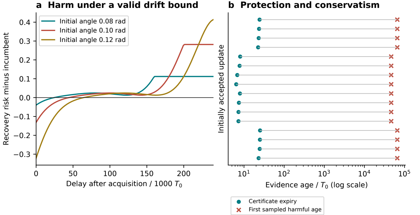
FIG. 3. Timing prevents harmful reuse under a valid drift premise, with conservative expiry. (a) Exact-channel excess recovery risk for the initially preferred correction after a continuous rate-limited ramp from three positive initial angles; negative-angle counterparts obey the same symmetry. Each point gives the recovery risk when the angle is held fixed during deployment at the value reached after the preceding drift. Positive excess risk denotes harm. The rate is 10^{-6} rad/ T_0 ; the ramp stops at the opposite initial angle. Acquisition precedes the ramp and deployment follows it. (b) Each row is one of the 16 independently sampled acquisitions initially admitted by confidence. Circles mark the end of the certified validity period; crosses mark full acquisition-to-completion age at the first harmful point on the 1500T_0 delay grid. Their separation exposes conservatism, rather than estimating a sharp optimal validity period. The remaining 8 acquisitions are rejected initially. Calibration-only acceptance admits later harmful updates in all 16 rows; the full confidence-and-timing rule rejects them. No drift assumption is violated.
