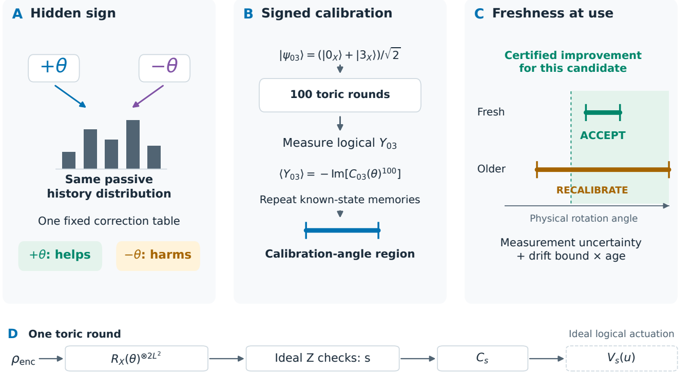
FIG. 1. Trusted calibration separates advice from authority over recovery. (a) Opposite rotation signs give identical passive syndrome-history distributions in the odd-distance square toric instrument defined in Sec. II, although one fixed correction table can help at one sign and harm at the other. (b) Known encoded calibration states undergo 100 rounds of the same toric instrument and a terminal logical Y_{03} measurement. Their sign-sensitive response supplies the missing observation; finite counts constrain the calibration angle. (c) The evaluator admits a proposed update only when sampling uncertainty and a justified drift bound certify recovery improvement at deployment; otherwise, the controller retains the incumbent or requests new calibration. The adviser can propose an action, including one induced by attacker-controlled text; the independent criterion determines whether that action may be applied. The displayed intervals are schematic. (d) The toric cycle uses ideal checks and X recovery C_s ; the dashed V_s(u) applies the specified logical operation without additional error. Circuit definitions are in Supplemental Material, Sec. V; the encoded calibration protocol is in Sec. Y. Figure 2 gives quantitative evidence for the complete chain.
