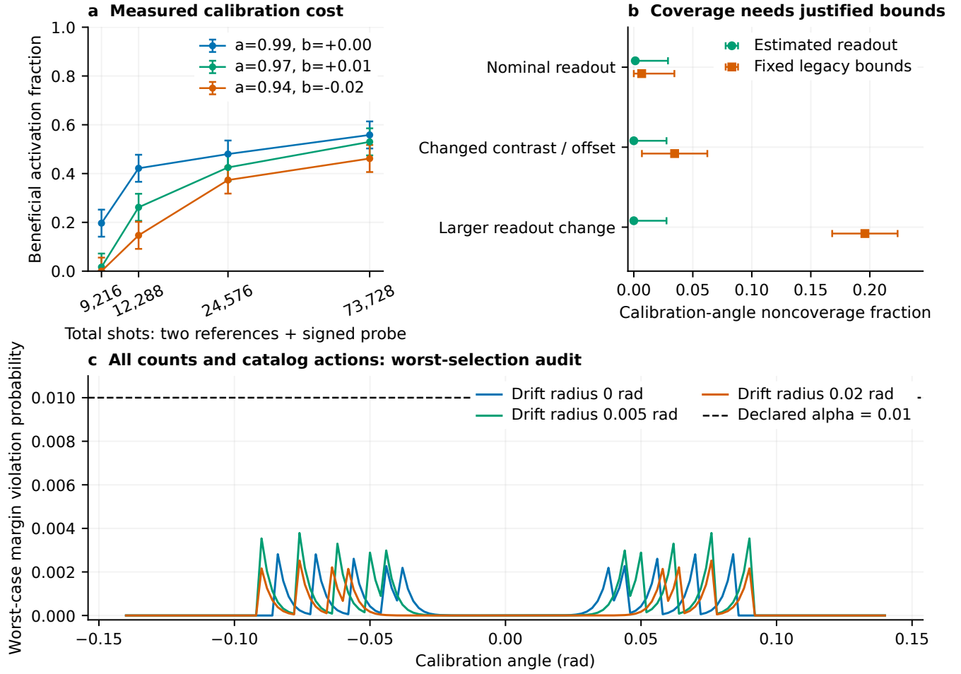
FIG. S20. Readout estimation trades shot cost for justified acceptance. Known-state references and signed-probe counts are simulated. (a) Beneficial-activation fraction versus total reference-plus-probe shots, using 600 independent records per cost point and readout setting. (b) Calibration-angle noncoverage for measured and fixed nuisance procedures, using 2400 records per setting. Panels (a,b) show pointwise 95% Hoeffding intervals. The changed readout settings violate the fixed procedure's nuisance assumptions. (c) Worst-selection margin-violation probability across the 5076-setting audit, maximizing over nuisance parameters and deployment shifts at each angle. Every possible 8192-shot count and all 13 catalog actions are evaluated. These curves sum binomial probabilities on a finite physical grid using the stated numerical treatment; they carry no sampling error bars. The dashed line is the declared \alpha = 0.01 .
