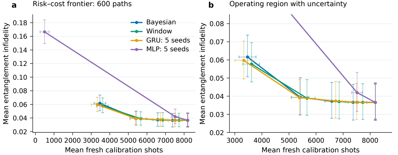
FIG. S7. Risk and calibration cost on 600 held-out simulated noise paths. The 5 evaluated prices per method are connected by visual guides. Horizontal and vertical bars show the saved pointwise hierarchical bootstrap 95% intervals for mean new calibration shots and infidelity. Neural methods are gated recurrent units (GRUs) and multilayer perceptrons (MLPs), each with 5 training seeds. The right panel expands the operating region. The horizontal axis counts new calibration shots beyond the common 3072 historical shots per path.
