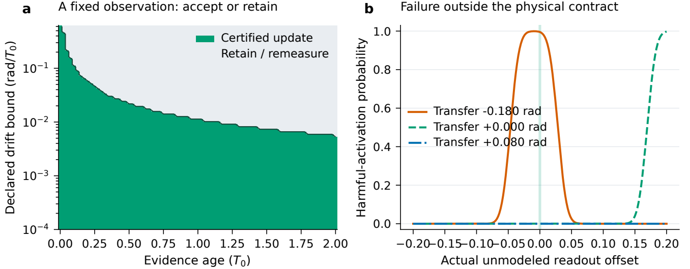
FIG. S6. Physical validity of the acceptance contract. Left: the acceptance region on an 81-by-81 grid of evidence ages and declared drift rates for one fixed observed block. Right: exhaustively summed binomial probabilities of harmful activation across 201 simulated offsets and selected transfer mismatches. The shaded offset band is the declared interval. Transfer outside \pm 0.001 rad violates the contract even at zero offset.
