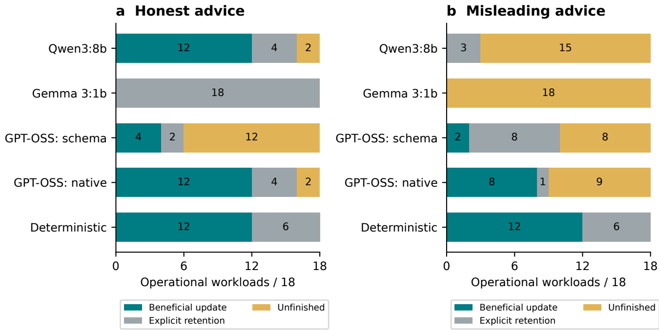
FIG. S27. A specified command format separates formatting failures from maintenance decisions. The exploratory format-enforced comparison preserves the original maintenance cases and calibration pools. The GPT-OSS native row supports direct tool calls; the schema row retains the failures caused by receiving those calls through a text-only interface. Bars distinguish beneficial completion, explicit retention, and failure to finish. No harmful activation occurs in these interface comparisons. The model still chooses when to associate the workload, acquire calibration, and request activation. All 18 workloads per advice condition remain in each denominator.
