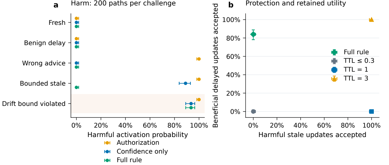
FIG. S4. Harm and utility in paired mechanism stress tests. (a) Harmful-activation fractions and pointwise exact 95% binomial intervals, 200 paths per case; the shaded case violates the drift premise. (b) The same stale-harm and benign-delay acceptance endpoints for the full rule and fixed expiry, with pointwise intervals on both axes. Time-to-live (TTL) values 0, 0.1, and 0.3 coincide. The benign-delay and bounded-stale challenges use different declared drift contexts.
