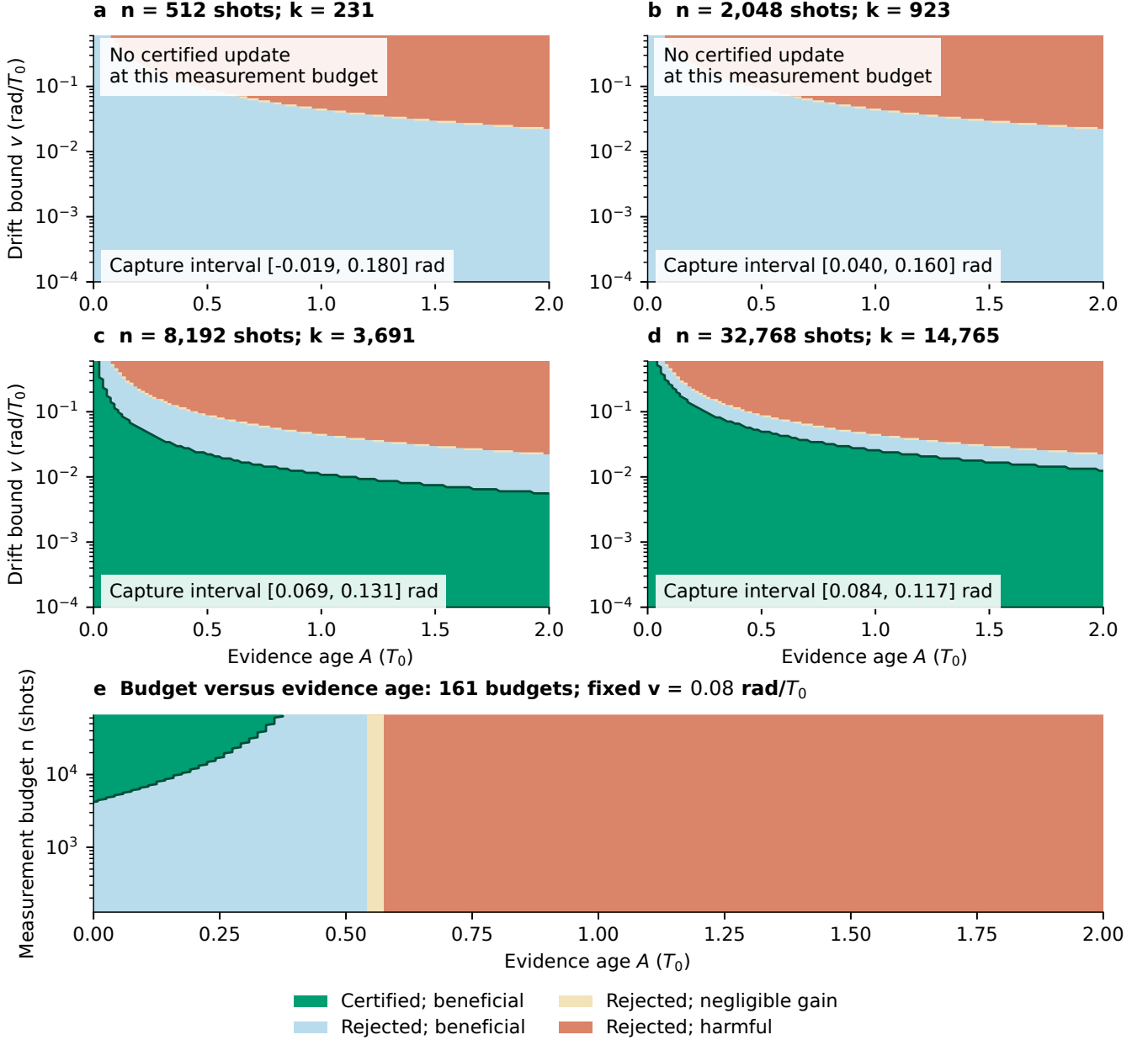
FIG. S12. Certification depends on measurement budget, evidence age, and drift. (a–d) Conditional decision maps at 4 shot budgets. (e) Budget–age section at v = 0.08 . Colors distinguish certification from the evaluator’s simulated outcome classification. Rejected beneficial updates quantify foregone opportunity: the controller must recalibrate, select another justified action, or retain the incumbent. The methods above specify the representative records and deployment path.
