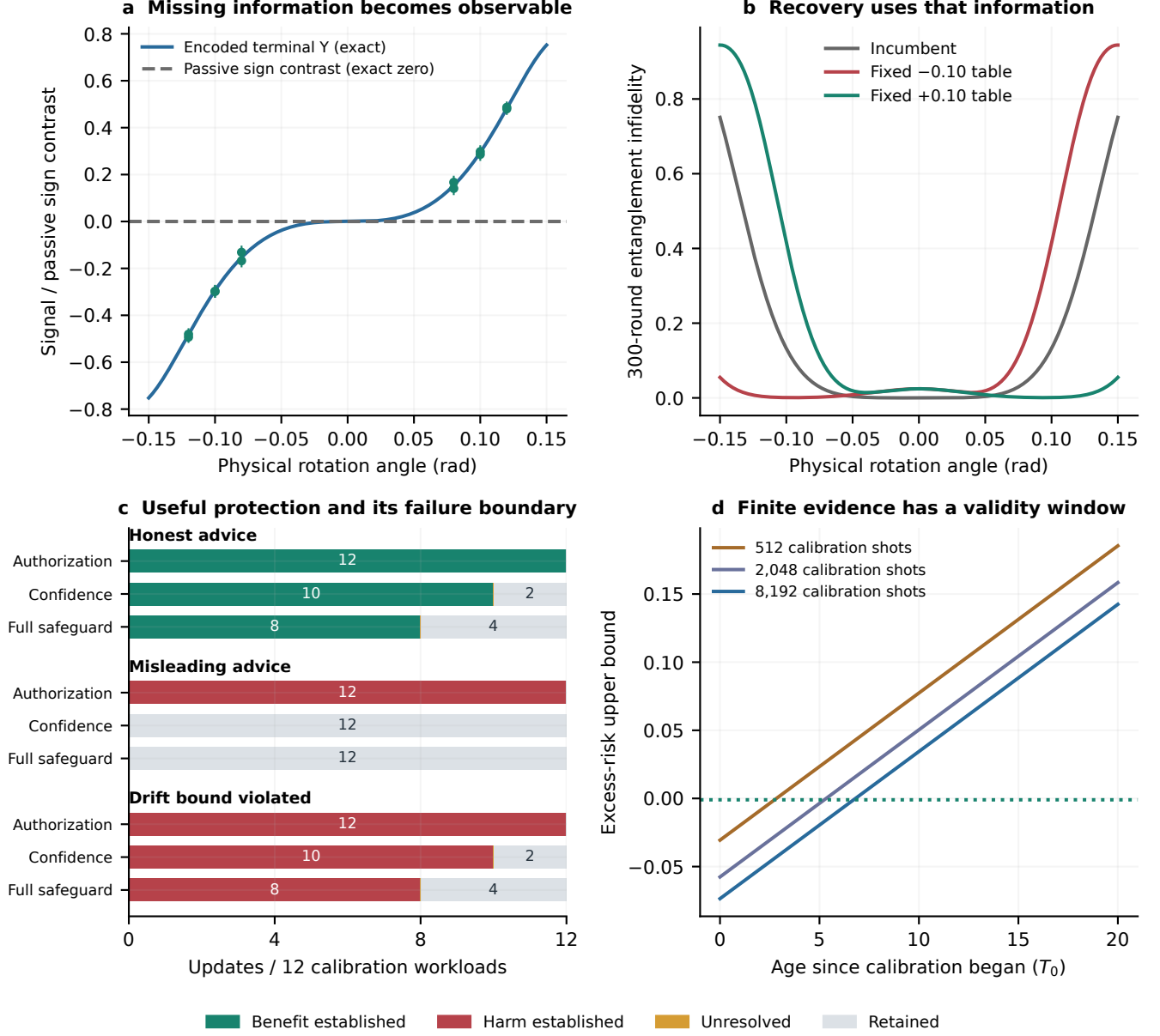
FIG. S24. Supporting response, recovery and timing calculations for the unified toric model. (a) Numerically evaluated encoded terminal signal and passive sign contrast, with the 12 8192-shot calibration records. (b) Stationary 300-round entanglement infidelity for the incumbent and fixed recovery tables at \pm 0.10 rad. The horizontal axis is the physical rotation angle; the vertical axis is recovery risk. (c) Aggregate outcomes for the same Qwen proposals under three rules; the invalid-drift condition violates the physical premise. (d) Upper bounds U_u^{\text{cal}} + L_D v A versus evidence age for 3 nested budgets in 1 calibration realization. Straight segments follow directly from the stipulated drift allowance. The curves illustrate this sufficient criterion; they do not measure the physical onset of harm. The full protocol is in Supplemental Material, Sec. Y.
