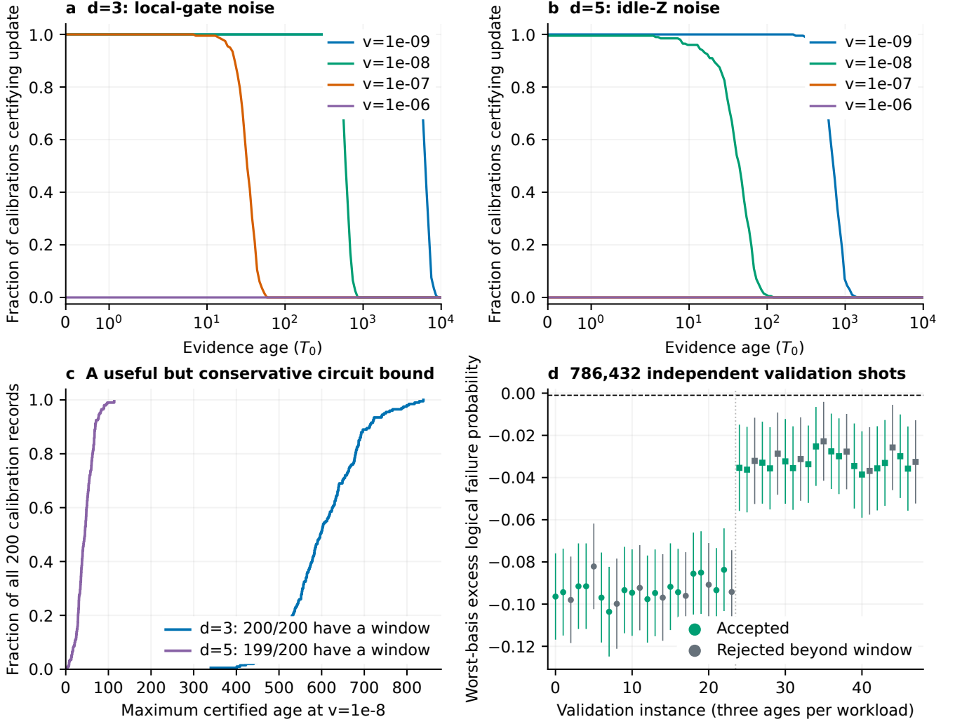
FIG. S22. Freshness within a specified scalar circuit-noise family. (a,b) Fraction of 200 reused calibration records per distance certifying an update at each age and declared drift rate. (c) Maximum certified deployment age at v = 10^{-8} per T_0 , retaining denominator 200 even when no window exists. (d) Independent final excess-risk estimates and conservative pointwise 95% intervals; circles and squares denote distances 3 and 5. Three ages share each of 8 calibration workloads per distance. Each instance uses 8192 shots per memory basis. All 48 intervals support benefit, including 16 updates rejected beyond expiry. The dashed line marks the required -0.001 improvement. Distance and noise family differ between the two circuit ensembles.
