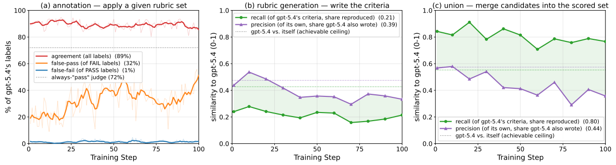
Figure 9: The three jobs a judge does, self-model vs. GPT-5.4 , measured by replaying the run’s judge calls through the policy checkpoint on the archived prompts, with a single call and no thinking (the ablated self-judge of Table 7). (a) Scoring a rubric it is given. How often the self-model returns the same verdict as GPT-5.4, over all 60,689 verdicts, and the two ways it can differ. Each series has its own denominator, named in the legend. Faint lines are per-step values, bold lines smoothed. (b) Writing the criteria and (c) merging them into the set a group is scored on. Here the two models write their own criteria, so we compare the sets themselves: a third model pairs up criteria that mean the same thing, and we then ask how much the two sets overlap. Recall is how much of GPT-5.4’s set the self-model also wrote; precision is how much of the self-model’s set GPT-5.4 also wrote. Legends give means, and the shading is simply the gap between the two curves. Perfect overlap is not the target, because two judges writing criteria for the same task will not pick the same checks: the dotted lines show GPT-5.4 compared against itself on two rollouts of one task, and are the reference to read the curves against. The self-model scores a given rubric well but too leniently, reproduces only about a fifth of the criteria GPT-5.4 writes, and at the merge keeps most of GPT-5.4’s criteria while adding roughly twice as many of its own.
