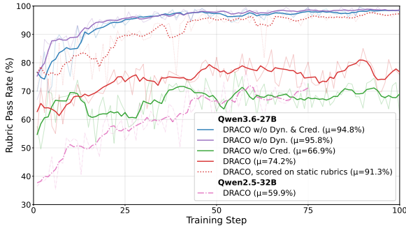
Figure 4: Overall rubric pass rate across training steps. Each setting is evaluated on its training rubrics (dynamic rubrics vary per step). The dotted line shows DRACO re-scored on the static held-out rubric set. Figure 10 in Appendix A reports per-criterion pass rates.
