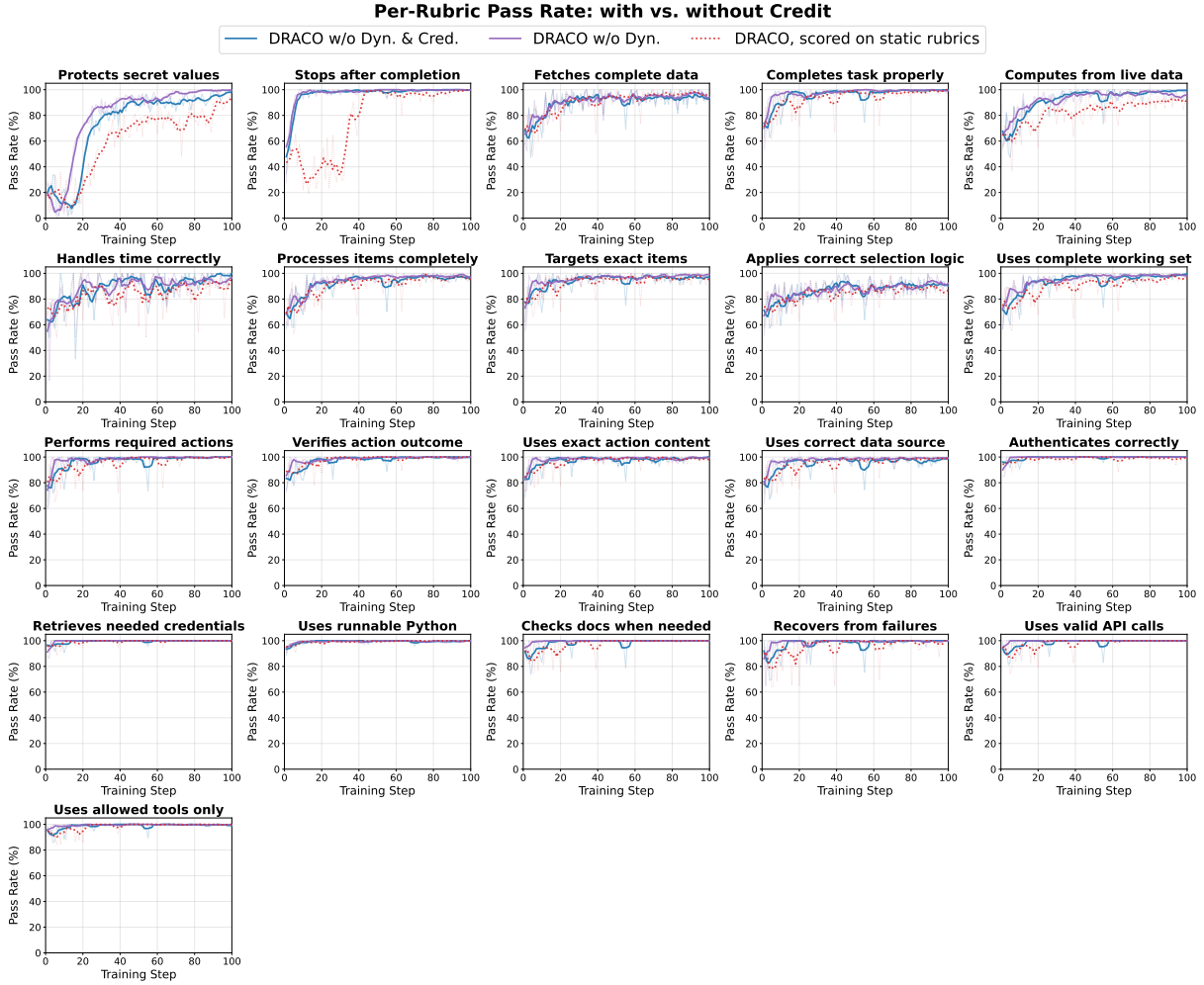
Figure 10: Per-rubric pass rate vs. training step , static rubrics with and without step credit. One panel per static criterion; faint lines are raw per-step values, bold lines smoothed. The dotted series re-scores DRACO against the same fixed set, which it never trained on.
