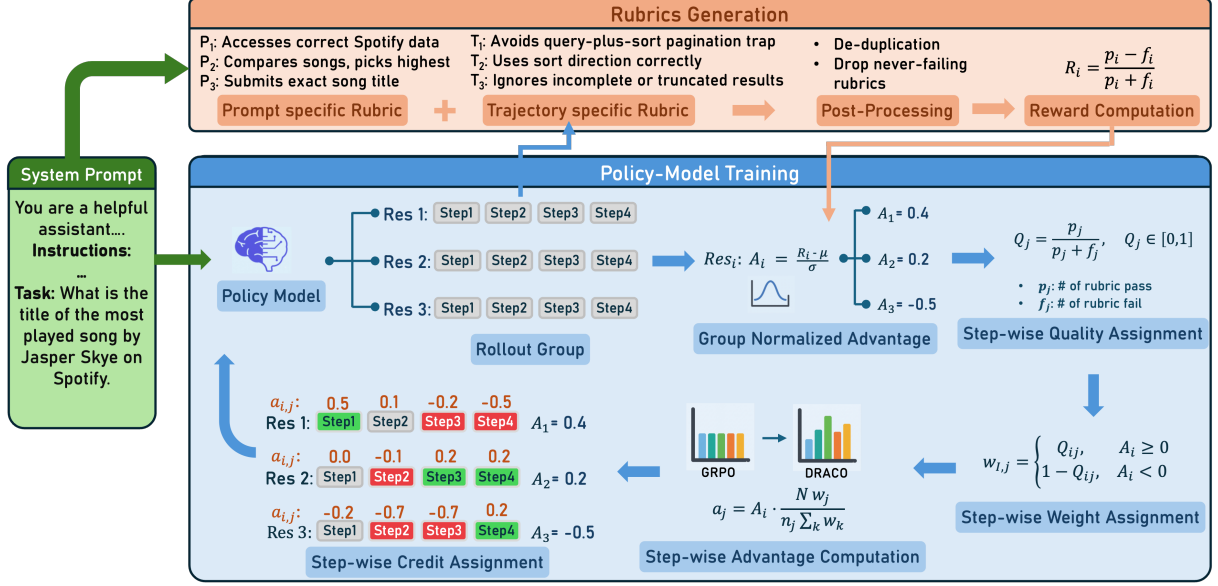
Figure 1: Overview of DRACO. Top: for each task, the judge proposes criteria from the instruction and each sampled trajectory; proposals are merged, deduplicated, and scored to produce an outcome-blind reward R_i (Section 3.2). Bottom: within a rollout group, GRPO normalizes rewards into trajectory advantages A_i ; DRACO then reallocates each A_i across steps according to the judge’s per-criterion verdicts, yielding step advantages a_j that concentrate credit on the steps the rubric implicates (Section 3.3).
