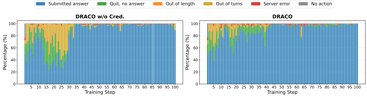
Figure 3: Rollout termination modes across training steps for DRACO with and without step credit. Bars show the percentage of rollouts per termination mode (normal completion/give-up vs. length, turn, or server errors), independent of task correctness. We interpret broad trends rather than exact error distributions.
