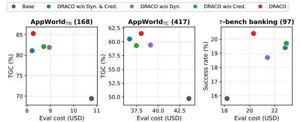
Figure 2: Performance vs. evaluation cost , one panel per benchmark; up and to the left is better. AppWorld panels plot TGC, \tau -bench banking plots success rate; SGC follows the same ordering (Table 2). Cost is the US-dollar total for one pass over the full split at the rates of Section 4.1.3; the \tau -bench axis also includes the GPT-5.4 user simulator and judge. Points are Qwen3.6-27B p^1 values from Table 2.
