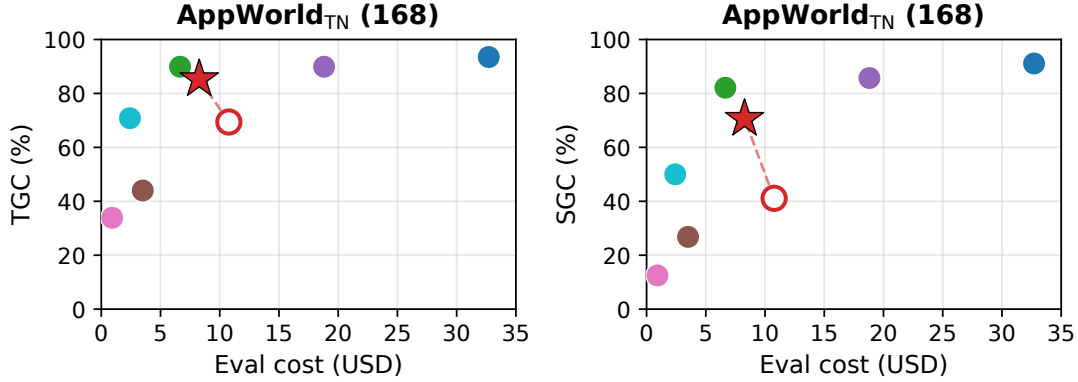
Figure 6: Frontier models vs. DRACO on AppWorld TN . TGC (left) and SGC (right) against the cost of one pass over the 168 tasks; up and to the left is better. Circles: frontier models, one run each. Star: DRACO on Qwen3.6-27B with the frontier judge. Hollow circle: the same policy untrained. Brackets give parameter counts (total, active) for open-weight models; closed models publish none. Values are in Table 8.
