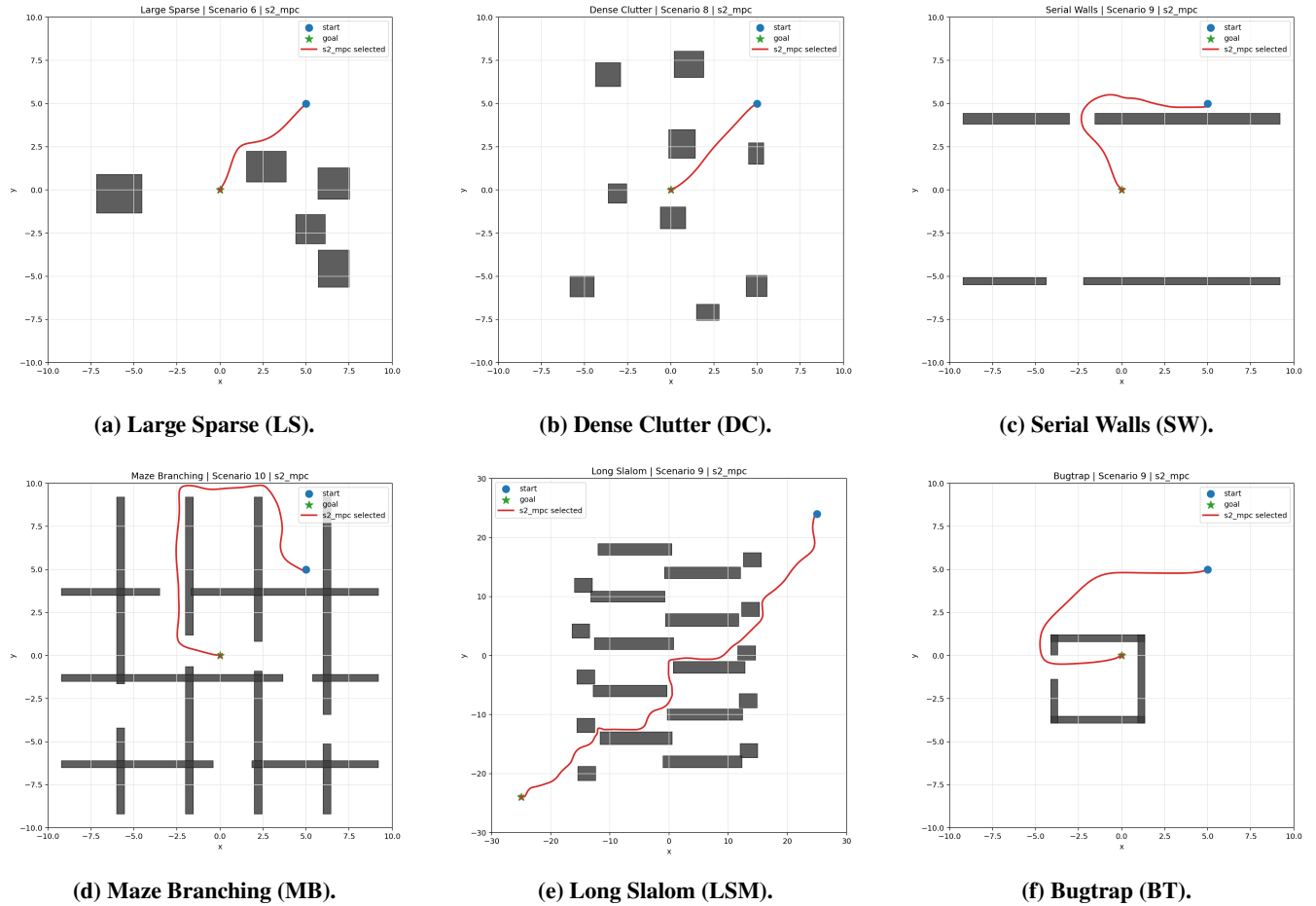
Figure 4: Representative nonlinear motion-planning environments used in the evaluation. Each panel shows an example map from one benchmark family.
