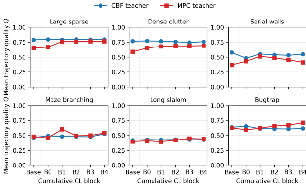
Figure 2: Mean quality Q of successful S1 rollouts on the 500-instance probe set as continual learning accumulates experience. Quality is evaluated only on successful rollouts.
