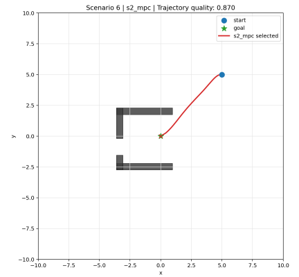
(c) S2-MPC. Q = 0.870 .
