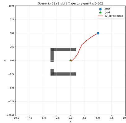
(b) S2-CBF. Q = 0.802 .
