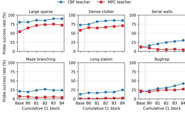
Figure 1: Success rate of S1 on the 500-instance probe set as continual learning accumulates experience. Solid curves show the CBF- and MPC-taught policies.
