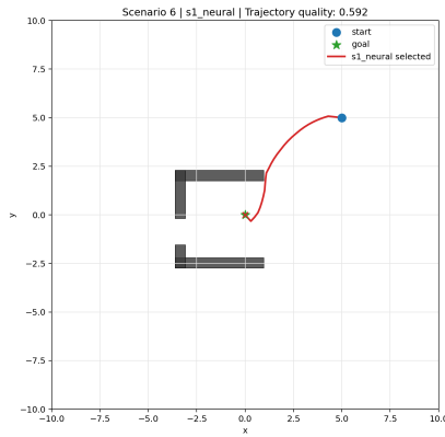
(a) S1-NN. Q = 0.592 .
