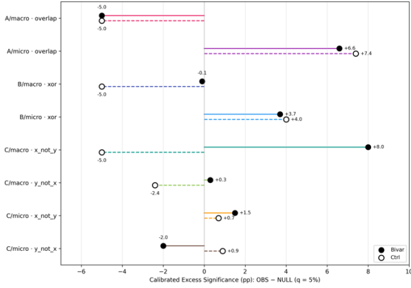
Figure 2: Calibrated excess significance (OBS – NULL, q = 5\% , percentage points) across representative operating points. Filled markers denote bivariate tests; open markers denote 4-speaker control; values < 0 indicate fewer rejections than the null baseline.
