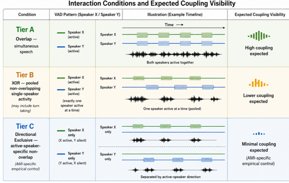
Figure 1: Interaction conditions and expected coupling visibility. Tier A denotes overlapping speech; Tier B pools non-overlapping single-speaker activity; Tier C separates that activity by active-speaker direction and is used as an AMI-specific empirical control.
