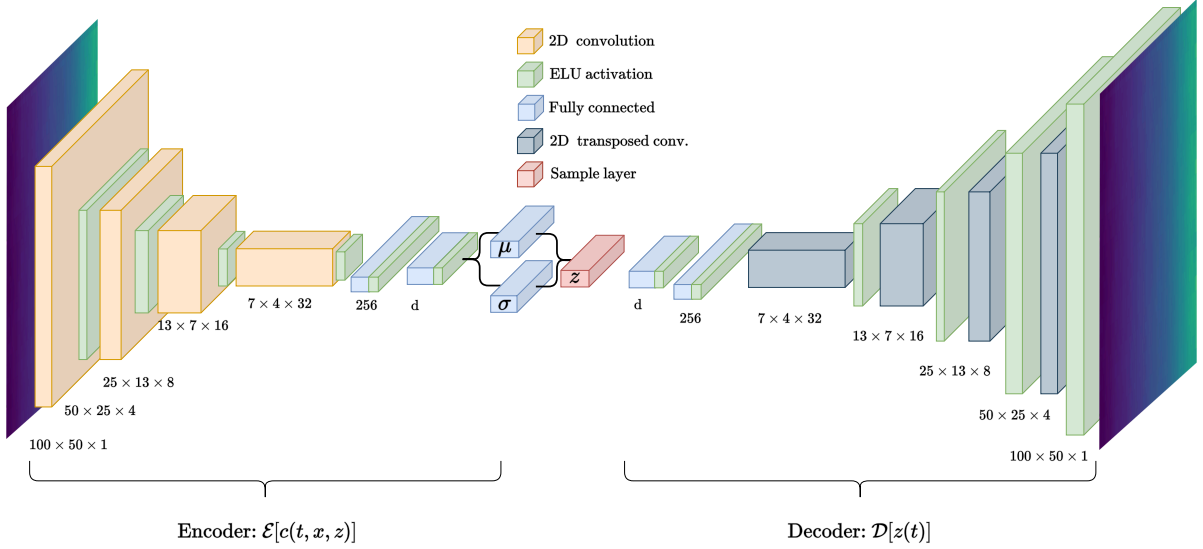
Figure 2: Schematic representation of the encoding-decoding process. A high dimensional map c_{t_0}(x, z) at a given time point t_0 is taken and encoded onto its respective latent space representation z_{t_0} . It can then be decoded by propagating it through the decoder network \mathcal{D} , recovering the high dimensional representation \tilde{c}_{t_0}(x, z) , which should be as close to the original input as possible.
