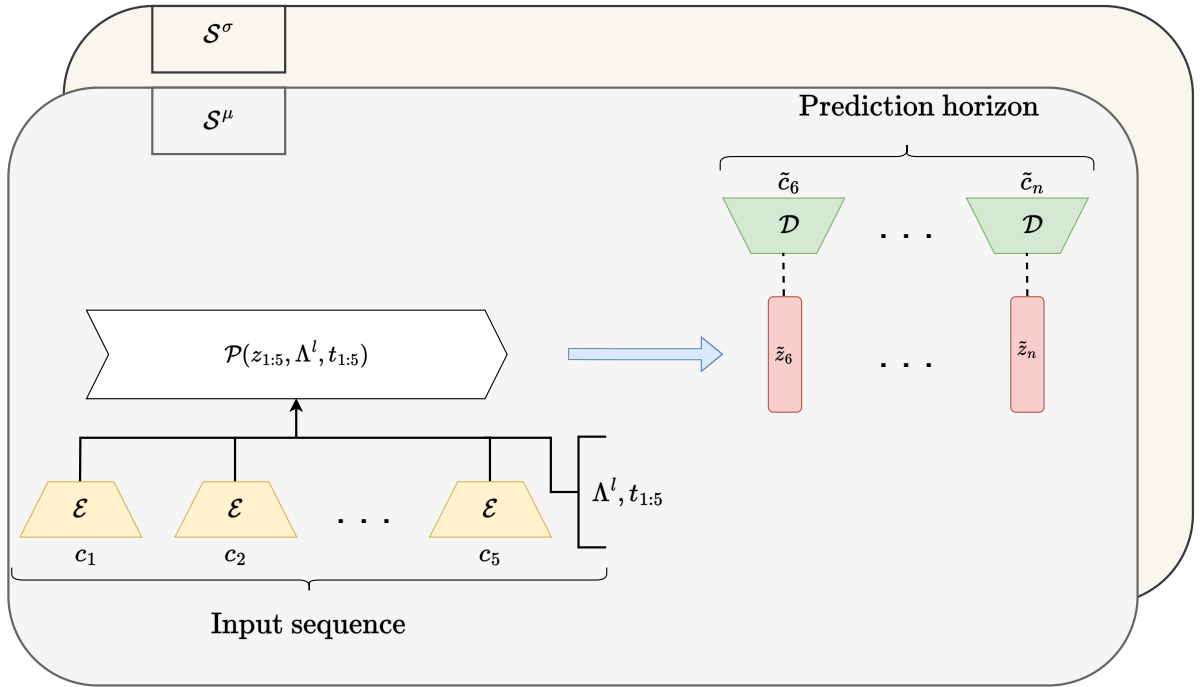
Figure 1: Visualization of the entire surrogate model using a multi-horizon forecasting model as the propagator \mathcal{P} . \mathcal{E} and \mathcal{D} are the encoder/ decoder parts of the VAE, c_i are the input configurations and \tilde{c}_i are the predicted next configurations. This process is repeated to predict sequences that are longer than the prediction horizon of the multi-horizon model. All the models have a \mathcal{S}^\mu branch that predicts the evolution of the dynamics. Stochastic models have an additional \mathcal{S}^\sigma branch that predicts the stochastic behaviour of the evolution.
