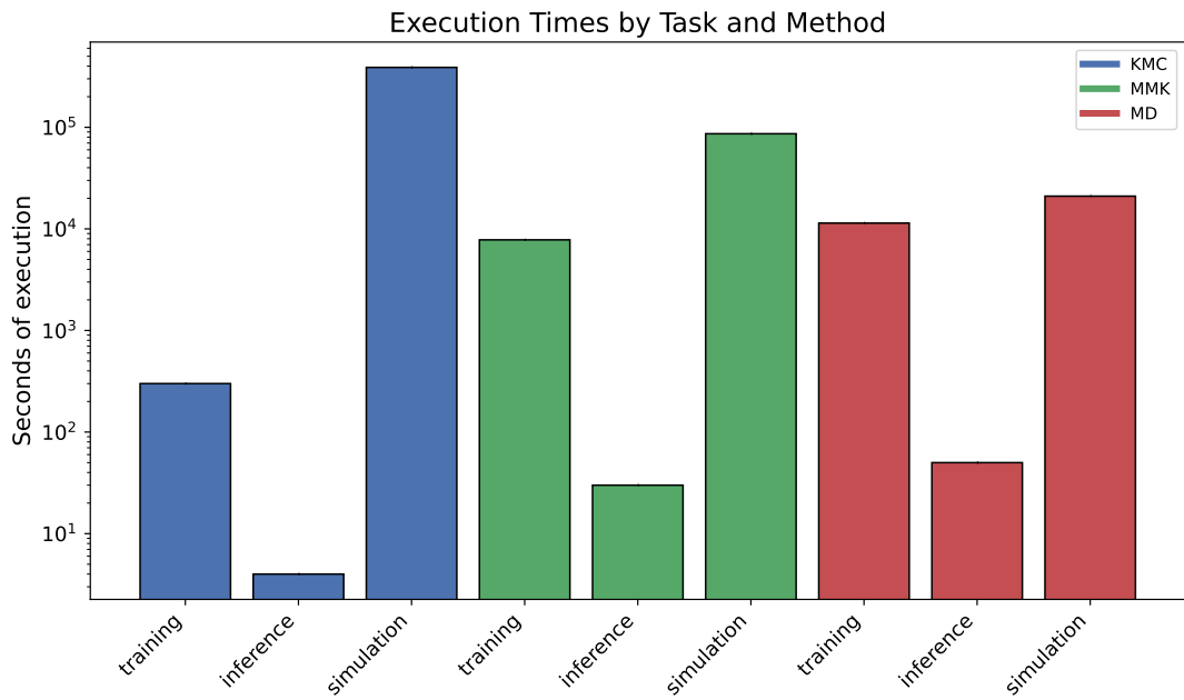
Figure 10: Time required for the execution of the simulation, the training of the model and the inference.
