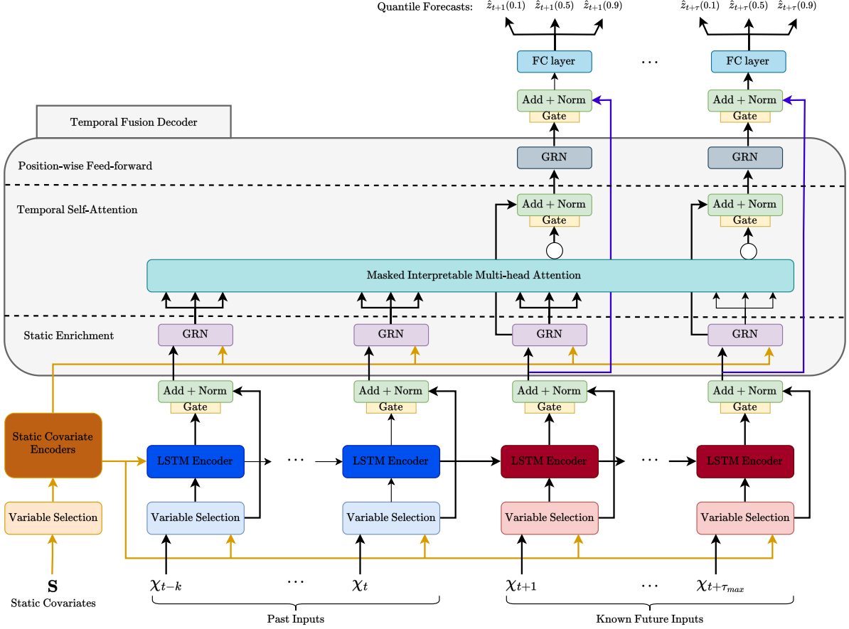
Figure 3: Temporal Fusion Transformer model, adapted from [33] Static covariates S and time-varying inputs — past observations ( x_{t-k} \dots x_t ) and known future covariates ( x_{t+1} \dots x_{t+\tau_{max}} ) enter through dedicated Variable Selection Networks (orange), which learn instance-wise feature weights for interpretability. The Static Covariate Encoder (dark orange) produces four context vectors used throughout the network: one for variable selection, two to initialize the LSTM’s cell/hidden state, and one for static enrichment. A sequence-to-sequence LSTM Encoder–Decoder (blue = past, dark red = future) provides local temporal processing, replacing standard positional encoding. Every sub-block is wrapped in a Gate + Add and Norm unit (yellow/green), a GLU-based residual gate that lets the network skip unused components. LSTM outputs are enriched with static context via a Static Enrichment GRN (purple), then passed to Masked Interpretable Multi-Head Attention (teal), which lets each time step attend to relevant past and future points while preserving causal masking. This is followed by a Position-wise Feed-Forward GRN, another gated residual block, and a final FC layer producing quantile forecasts ( \hat{z}_{t+\tau}(0.1) , (0.5) , (0.9) ) at each horizon step — enabling calibrated uncertainty estimates alongside point predictions.
