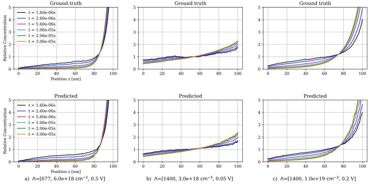
Figure 5: Predictions of the surrogate model for the mean field of the three different parameter configurations a)-c). The combination of parameters strongly affects the final concentration profile as well as the dynamic process that precedes the steady-state concentration distribution. The time stamps correspond to the following list of time steps: [10, 20, 50, 100, 200, 300]. The representation shows the evolution of the concentration summed up along the Z axis and averaged over multiple simulation runs.
