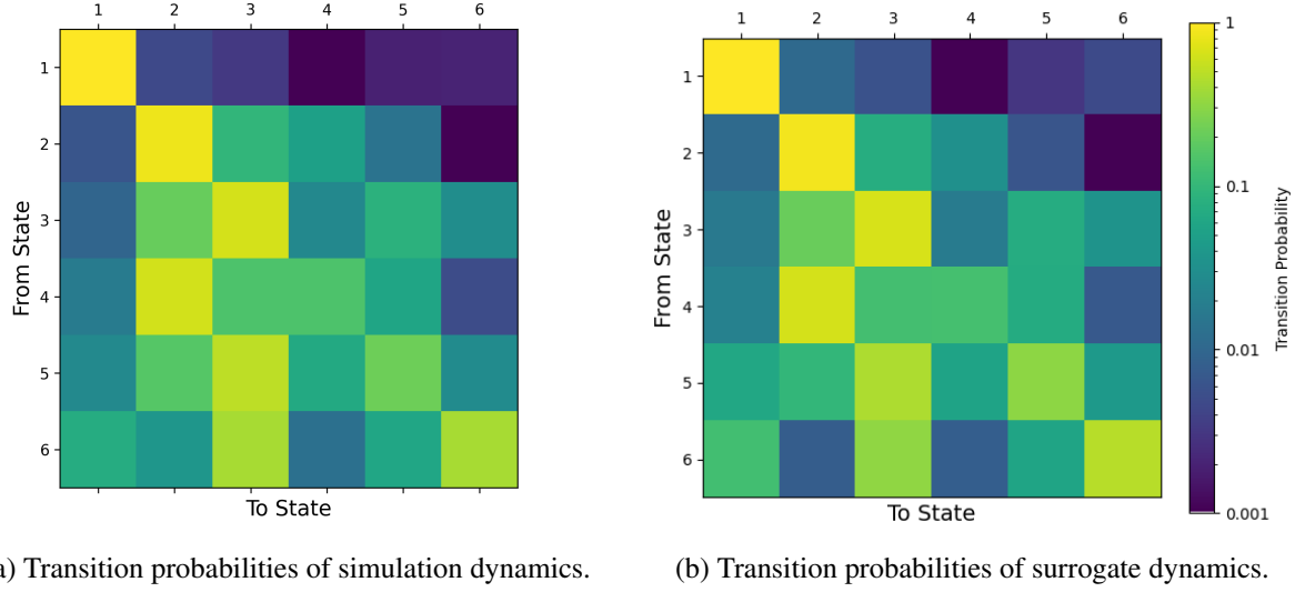
Figure 9: Comparison of Transition probabilities between simulation and surrogate dynamics. States labeled in fig. 8
