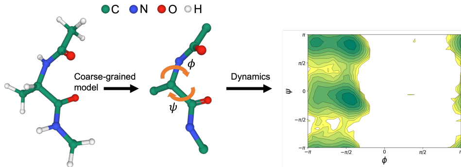
Figure 7: The system used for surrogate of molecular dynamics. The hydrogens are removed from the MD configurations. The two ramachandran angle \phi and \psi are indicated.
