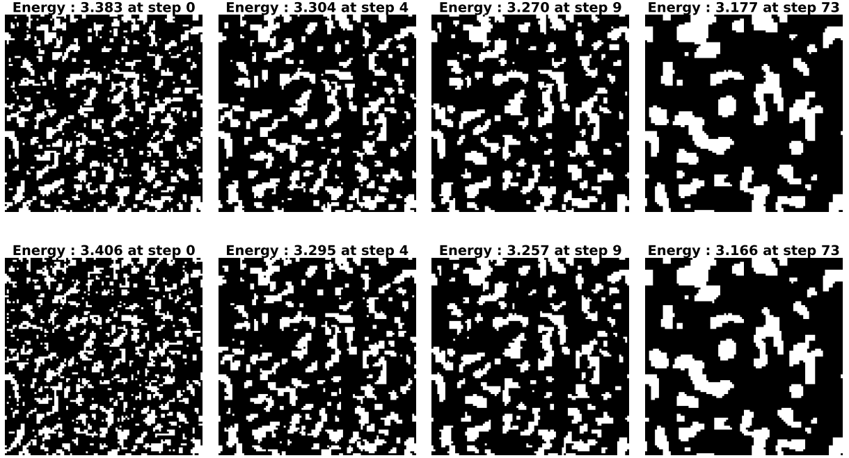
Figure 4: Snapshots generated through the physical simulation (up) and snapshots generated through our framework (down) with their energies and corresponding timesteps
