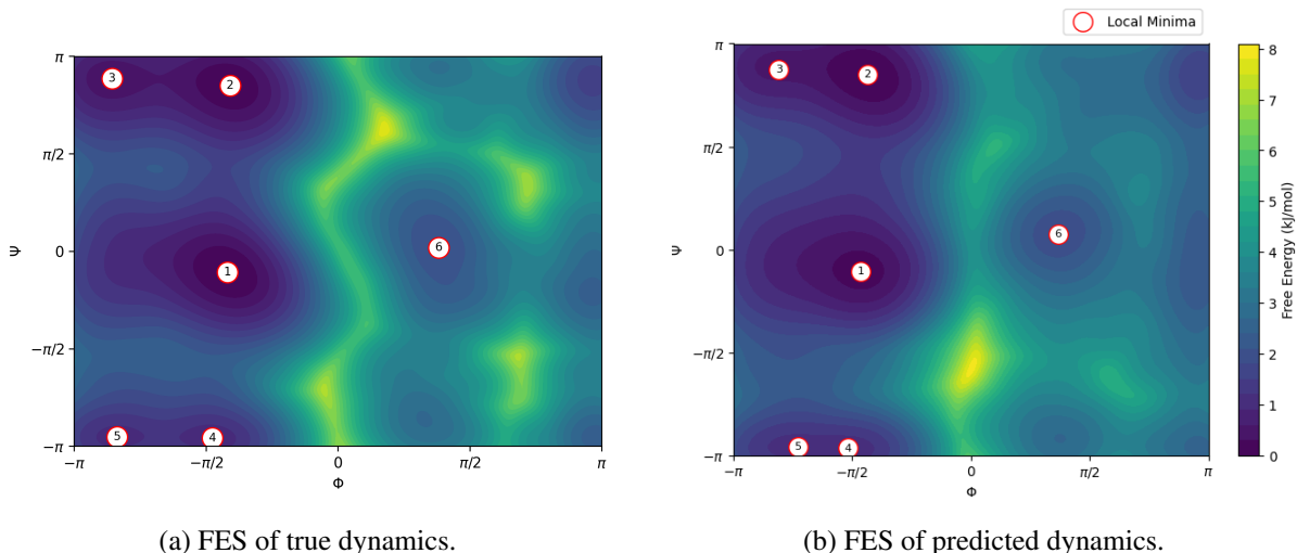
Figure 8: Comparison of Free Energy Surface (FES) of the dihedral angles \phi and \psi between true and surrogate dynamics.
