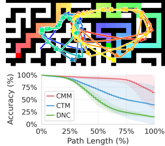
Figure 4: Top: CMM attention traces a path through the 39 \times 39 maze (crop). Bottom: Accuracy by maze path length. The CMM performs best on longer paths.
