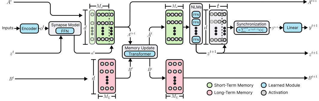
Figure 1: The Continuous Memory Machine. At timestep t , the current observation o^t and previous activated state z^t are processed by the feedforward synapse model to produce a pre-activated state a^t . This state is appended to the sliding short-term memory (STM) A^t . A^t and the long-term memory B^t are jointly processed by a Transformer, producing updated memories \tilde{A}^t and \tilde{B}^t . \tilde{A}^t is passed through the neuron-level models to produce the next activated state z^{t+1} . From the activated-state history, the model computes the synchronization S^{t+1} and output y^{t+1} . A^t , \tilde{B}^t = B^{t+1} , and z^{t+1} are carried forward to the next iteration.
