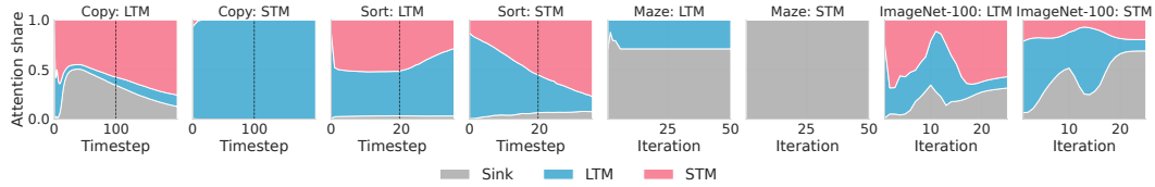
Figure 6: Memory attention across tasks. Each pair shows LTM queries (left) and STM queries (right), with attention to the sink, LTM, and STM tokens. CMM learns task-specific memory strategies.
