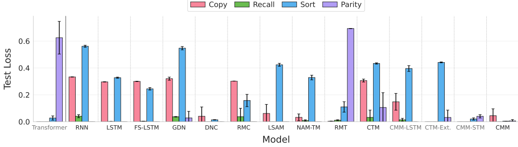
Figure 2: Loss for algorithmic tasks. The CMM demonstrates strong performance on all four tasks.
