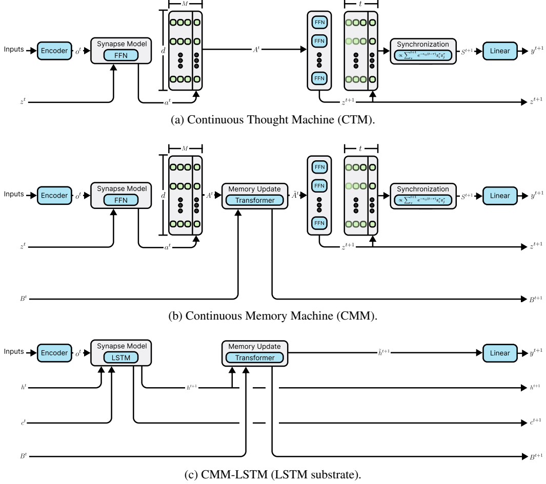
Figure 7: Comparison of the Continuous Thought Machine (top), the Continuous Memory Machine (middle), and CMM-LSTM (bottom). The CTM maintains a sliding short-term memory (STM) of recent pre-activations, which is processed by independent neuron-level models, while the synchronization module computes time-decayed outer products of activation histories that are projected to output logits. The CMM extends the CTM with a persistent long-term memory (LTM) that is jointly updated with the STM through the memory-update Transformer before the neuron-level models are applied. CMM-LSTM replaces the CTM backbone with a LayerNorm LSTM while retaining the same LTM and memory-update Transformer. Consequently, the Transformer receives a single hidden-state token instead of the CTM’s sliding window of M_S STM tokens, and there are no neuron-level models or synchronization representation. Comparing the CMM and CMM-LSTM isolates the contribution of the CTM’s distributed short-term representation and per-neuron processing.
