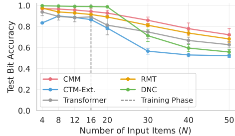
Figure 3: The CMM generalizes best on sort.
