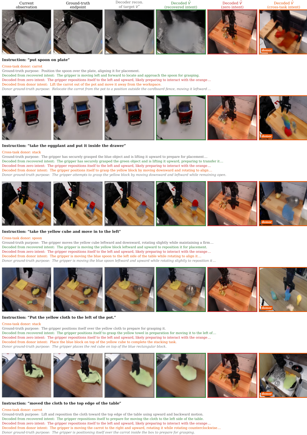
Figure 12: Learned visual and textual readout of intent. Each row shows the current observation, ground-truth endpoint, visual reconstruction from V_t^* , and visual outcomes decoded from \hat{V}_t under recovered, zero, and cross-task intent. The text below each row shows the ground-truth purpose and statements decoded from recovered, zero, and injected intent. Recovered intent produces an outcome and purpose consistent with the current behavior, while cross-task intent redirects both modalities toward the injected behavior.
