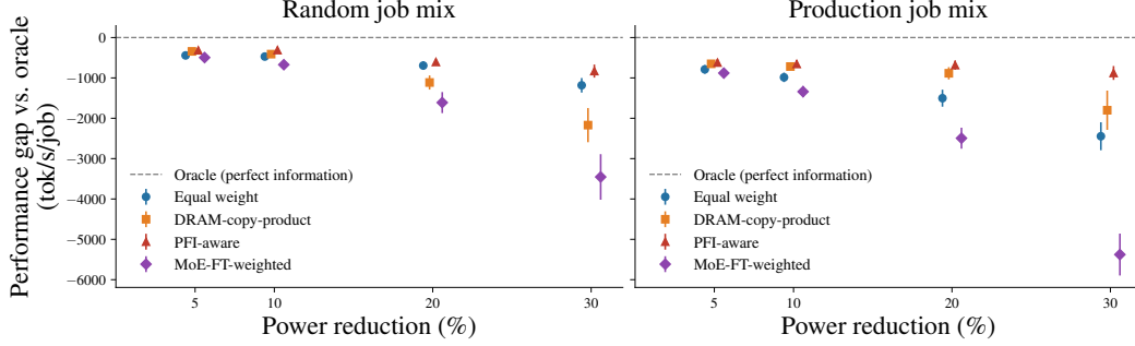
Figure 8: Difference in throughput for four allocation strategies compared against an oracle with perfect information of each job’s power-performance curve (less negative = closer to optimal) across a range of curtailment targets and workload mixes (random = jobs sampled at random from our dataset, production = jobs sampled according to the pretraining/fine-tuning mix from recent work [10]).
