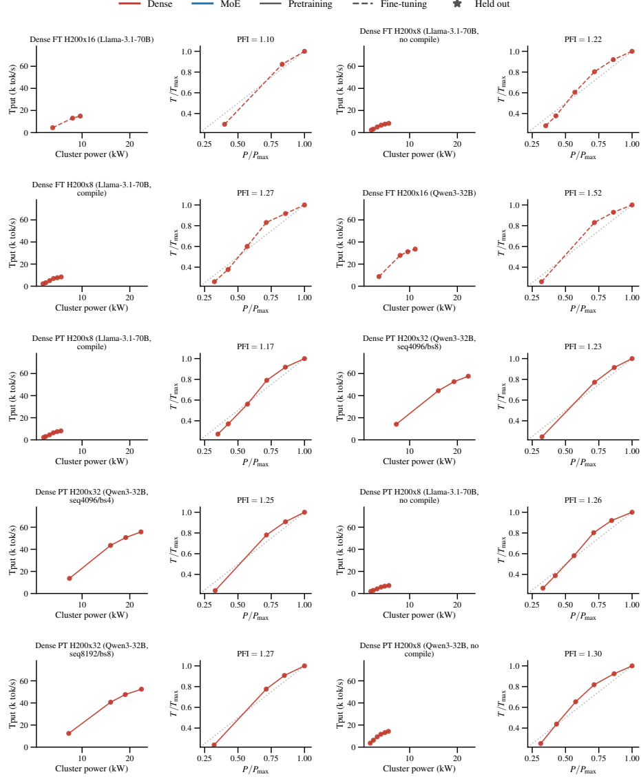
Figure 11: Power-throughput curves (raw and normalized) for each headline and validation run on H200.
