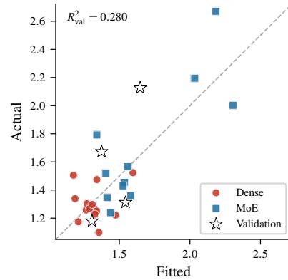
Figure 7: Predictions of the PFI model fit to DRAM copy product, including the validation set.
