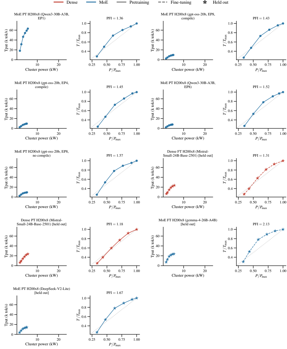
Figure 13: Power-throughput curves (raw and normalized) for each headline and validation run on H200 (continued).
