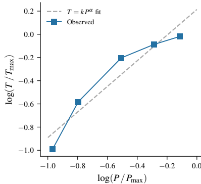
Figure 9: Comparison of constant-elasticity fit with the observed power-performance curve for gpt-oss-20b fine-tuning on 8 \times H200 s.
