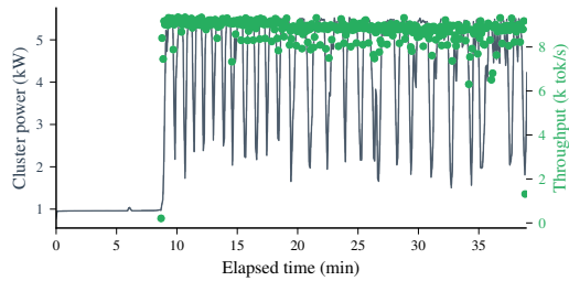
Figure 2: Aggregate GPU power and training throughput for a representative QWEN3-32B pretraining run on 32×H200 at 700 W/GPU.
