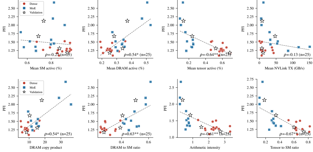
Figure 5: PFI vs. GPU telemetry metrics, showing the correlation (ordinary least-squares fit and Spearman \rho ) between PFI and metrics measured for the uncapped job in each sweep group. DRAM copy product and tensor to SM ratio are derived metrics. * q < 0.05 , ** q < 0.01 , where q is the Benjamini–Hochberg FDR-corrected p -value across all metrics tested in Fig. 14 in the appendix.
