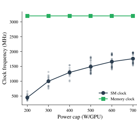
Figure 6: Steady-state SM clock and memory clock frequency as a function of power cap.
