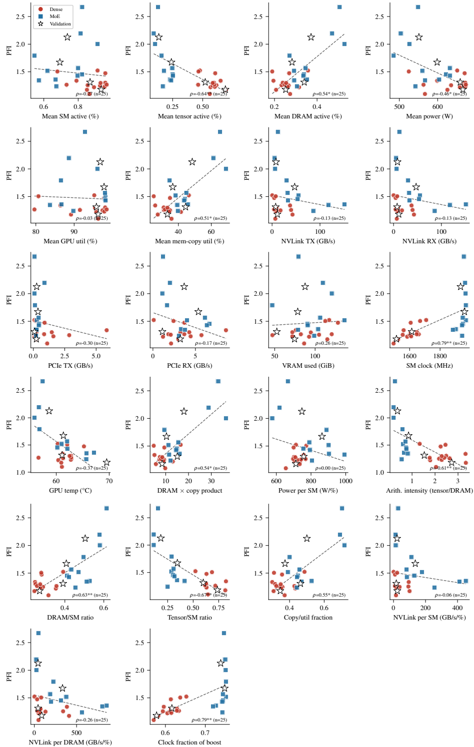
Figure 14: PFI vs. all DCGM GPU metrics and composite features. Dashed lines show ordinary least-squares fit; Spearman \rho and significance are annotated. ^*q < 0.05 , ^{**}q < 0.01 , where q is the Benjamini–Hochberg FDR-corrected p -value across all metrics in this figure.
