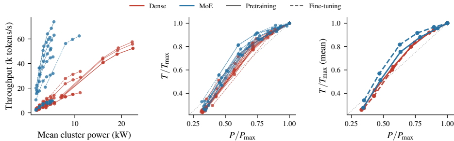
Figure 3: Power–performance curves for all sweep groups. Left: Aggregate GPU power vs. throughput. Center: Per-sweep normalized power vs. throughput. Right: Mean normalized power vs. throughput for each category (dense vs. MoE, pretraining vs. LoRA SFT). Full data are provided in Appendix C.
