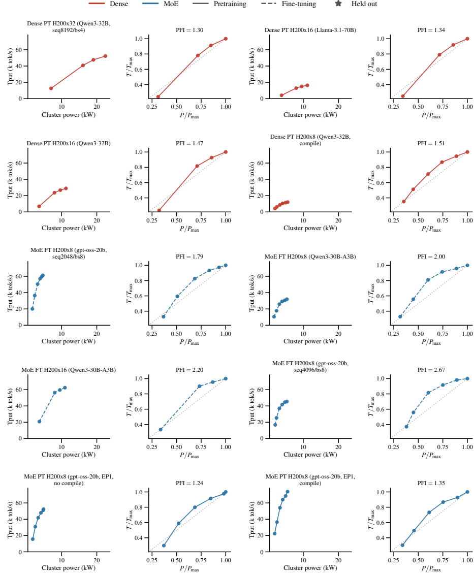
Figure 12: Power-throughput curves (raw and normalized) for each headline and validation run on H200 (continued).
