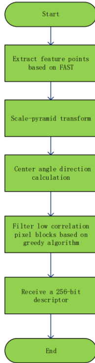
Fig. 4. ORB feature extraction and the matching flowchart.
