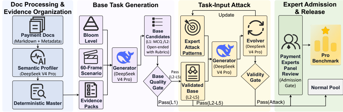
Figure 1: BENCHCOMPASS uses scenario-first evidence-pack construction. The system builds structure-aware chunks, semantic profiles, typed evidence packs, and grounded scenarios before generating questions.
