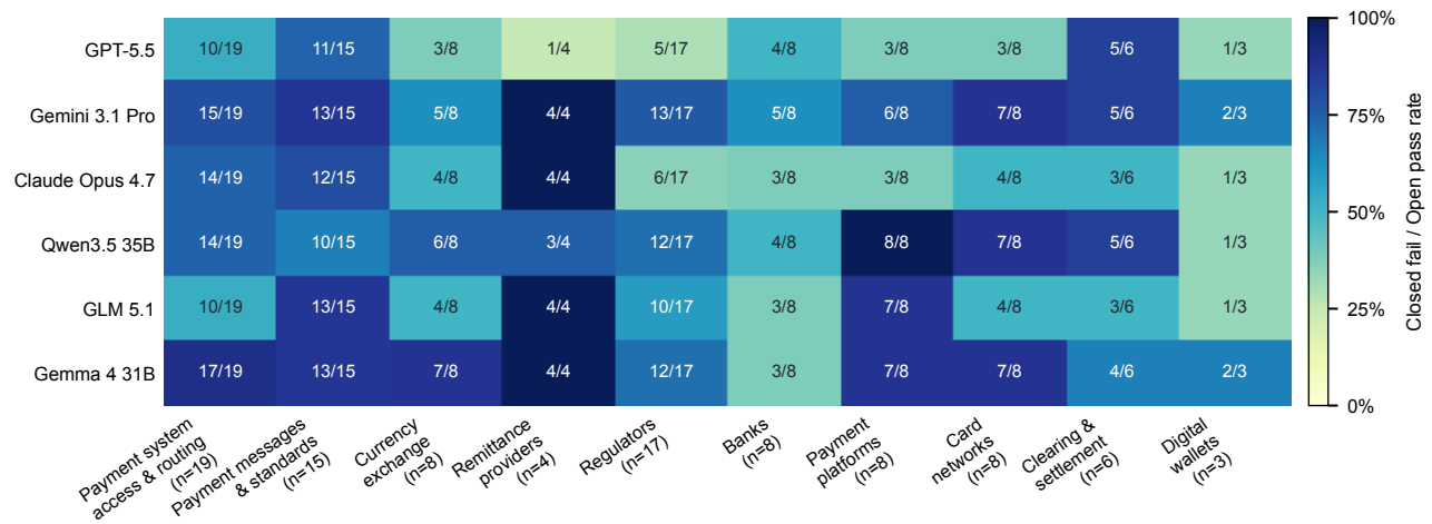
Figure 4: Where Open context rescues representative models. Each cell counts L2–L5 cases where a model fails Closed but passes Open, grouped by the case’s primary source category. Larger counts indicate source areas where the model lacks accessible parametric knowledge but can use the supplied source context.
