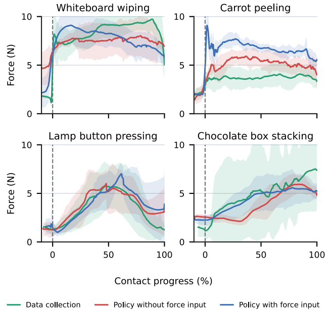
Fig. 6. Contact force for data collection (green), policy rollouts without force input (red), and policy rollouts with force input (blue), shown as mean \pm one standard deviation over in-contact task progress: the normalized end-effector path length accumulated during contact (0%: contact onset, dashed line; 100%: contact release), which factors out differences in execution speed and object placement across runs. We use all available data-collection executions and all successful policy rollouts.
