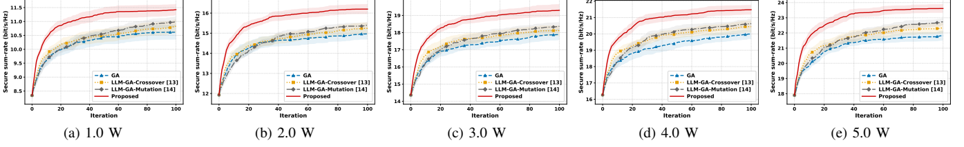
Fig. 3. Secure sum-rate convergence for five total transmit power levels.
