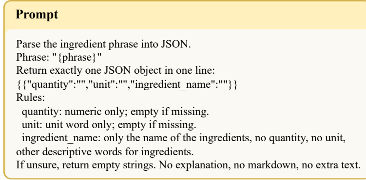
Figure 2. Prompt of component phrase analysis
