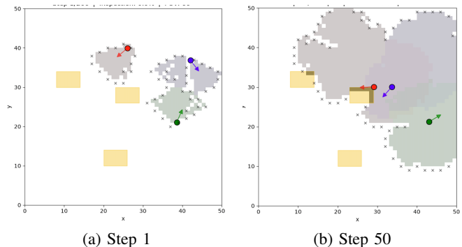
Fig. 1. Cooperative object inspection under partial observability. Agents with limited fields of view progressively reveal free space and inspection-object surfaces while coordinating their coverage.
