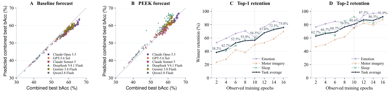
Figure 4. Early forecasts and candidate retention. (A–B) Ten-epoch forecasts versus actual combined validation bAcc for 269 architectures, averaging task-wise best-within-40 scores. (C–D) Top-one and top-two task-winner retention across observation windows; dark curves average the three tasks equally. Dotted lines mark ten epochs.
