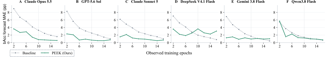
Figure 5. Forecast error across LLMs and observation windows. Combined validation bAcc MAE (pp), averaged over candidates within rounds and equally over paired rounds. Cohorts may vary by window; dotted lines mark ten epochs.
