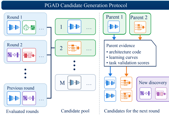
Figure 2. PGAD candidate generation protocol. Left: Architectures evaluated in previous discovery rounds. Middle: A shared candidate pool ranked by combined validation performance. Right: Top-ranked parents provide source code, learning curves, and task-specific validation scores for targeted refinements. These refinements are combined with fresh architecture proposals to form the next candidate batch.
