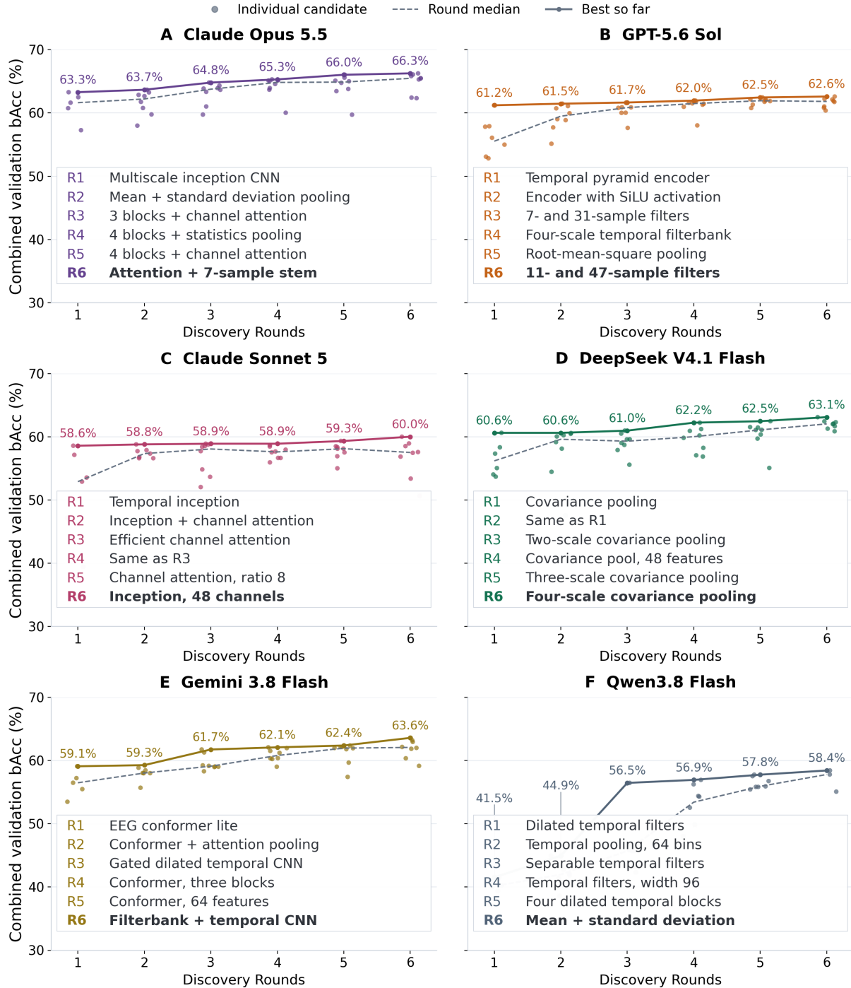
Figure 6. Architecture discovery with round incumbents. Dots show individual evaluated candidates; dashed and solid lines show round medians and cumulative best bAcc. Each inset names the incumbent after rounds R1–R6; bold text marks the final architecture.
