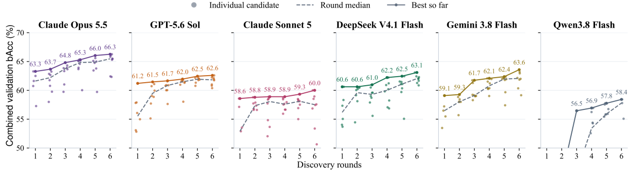
Figure 3. Discovery trajectories across six LLM-guided searches. Dots show candidates completed on all three tasks; dashed lines mark round medians, and solid lines track the best combined validation bAcc so far. Labels give the incumbent scores. The vertical axis is truncated at 50%; round-by-round architecture identities appear in Supplementary Figure 6.
