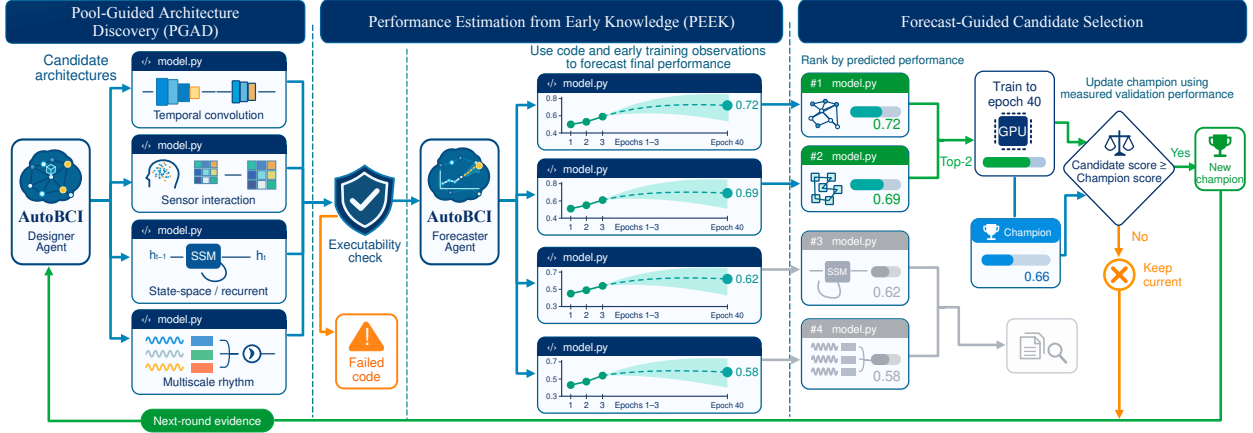
Figure 1. AutoBCI framework overview. The Designer Agent uses PGAD to generate and refine EEG architectures; the Forecaster Agent uses PEEK to predict performance and guide continued training. Validation feedback guides subsequent discovery rounds.
