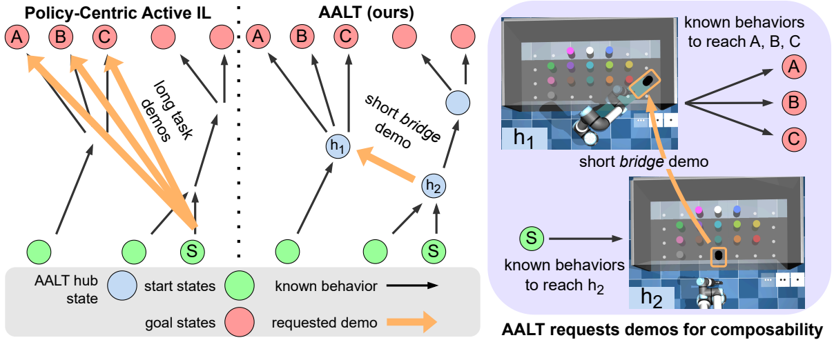
Figure 1: AALT requests demonstrations for composability. An agent begins with learned behaviors (black arrows) covering only some tasks between start states ( S ) and goal states ( A, B, C ), and may request additional expert demonstrations (orange arrows). (Left) Standard policy-centric active IL selects requests for their expected information about the expert policy. Because it does not explicitly value composability, it may request separate full-task demonstrations from S to A, B , and C , each of which may help the agent understand only one task. (Center) AALT instead organizes demonstrated behaviors into a topology connected through reusable latent hub states (blue), then requests short bridge demonstrations that maximize expected start–goal connectivity. Here, known behaviors reach h_2 , while other known behaviors lead from h_1 to A, B , and C . Requesting the bridge h_2 \rightarrow h_1 creates routes to all three goals with one short demonstration. During execution, the topology specifies a route through these hubs, while a learned policy generates actions from the current observations for each successive hub transition. (Right) In the simulated retrieval task, the bridge moves the black canister to transform h_2 into h_1 , from which the policy can pursue all three goals. Video of the simulation is provided in the supplementary material.
