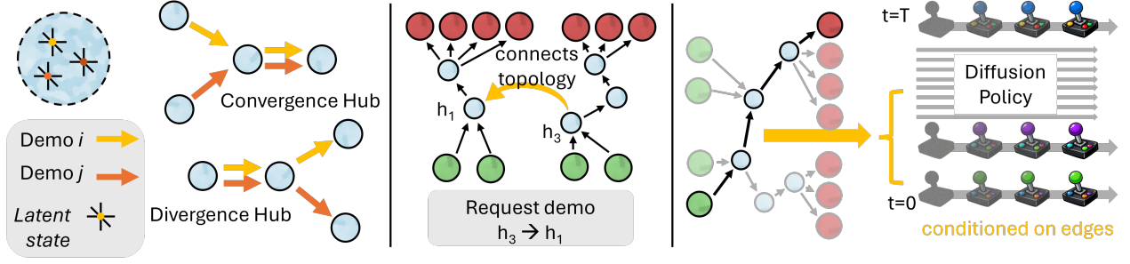
Figure 2: The AALT method. (Left) latent states are clustered, and may become hub states if they converge or diverge between different demos. (Center) hubs are linked by demos to form a topology of composable behaviors. New demonstration requests are selected to optimize start–goal connectivity. Here, h_3 \rightarrow h_1 would connect the right-side starts to the left side goals. (Right) during inference, we plan from the start state to a goal hub. A diffusion policy generates actions to reach the goal, conditioned on (h_i, h_j) from each edge.
