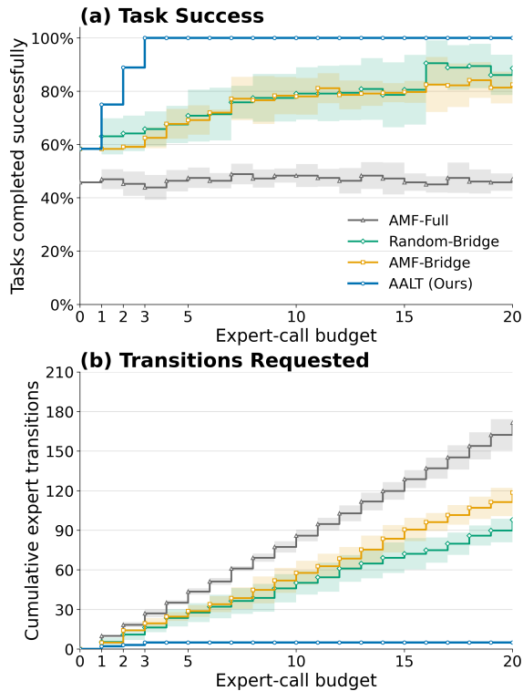
Figure 3: AALT solves all 72 tasks after only three expert calls totaling five transitions, whereas after 20 calls, the most effective baseline Random-Bridge reaches 88.6 \pm 9.9\% using 98.0 \pm 9.8 transitions. (a) Target-task success under increasing expert-call budgets ( \uparrow ). (b) Cumulative expert transitions requested ( \downarrow ).
