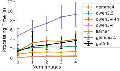
Figure 10: Inference efficiency for instruction-driven moderation by number of images in posts. gemini and gpt show high variance owing to API requests.
