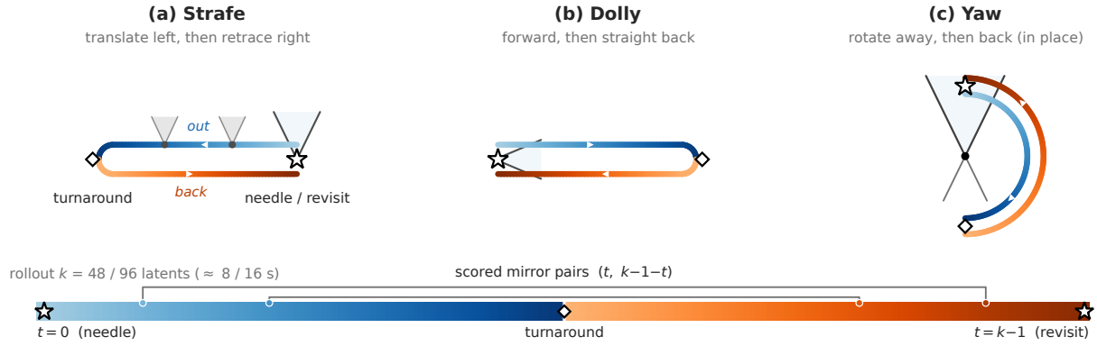
Figure 7 Constructed palindrome trajectories. The camera moves out (blue) and retraces its path (orange), so the needle view at t=0 must be regenerated at t=k-1 ; scored mirror pairs (t, k-1-t) span at least half the rollout.
