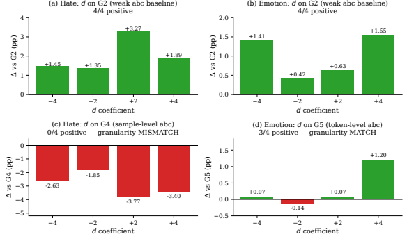
Figure 5: Gap signal d (single-seed sweep): positive in all 8 settings on the weak G_2 baseline (top row), while stacking on the task-best abc is granularity-conditional — emotion (token-level, MATCH): 3/4 positive; hate (sample-level, MISMATCH): 0/4 positive. Referenced from Section 4.4.
