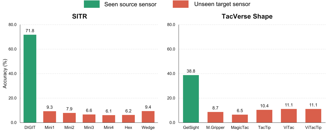
Figure 1: TVL performs well on the source sensor but collapses on unknown sensors. A linear classifier trained on the source sensor is evaluated with frozen TVL features and no target labels. Green bars denote seen source sensors and red bars denote unseen target sensors. Bars show mean accuracy over three seeds. On SITR, accuracy falls from 71.75% on DIGIT to 7.58% on average across six unknown sensors. On TacVerse Shape, it falls from 38.78% on GelSightNoMarker to 9.56% across five unknown sensors.
