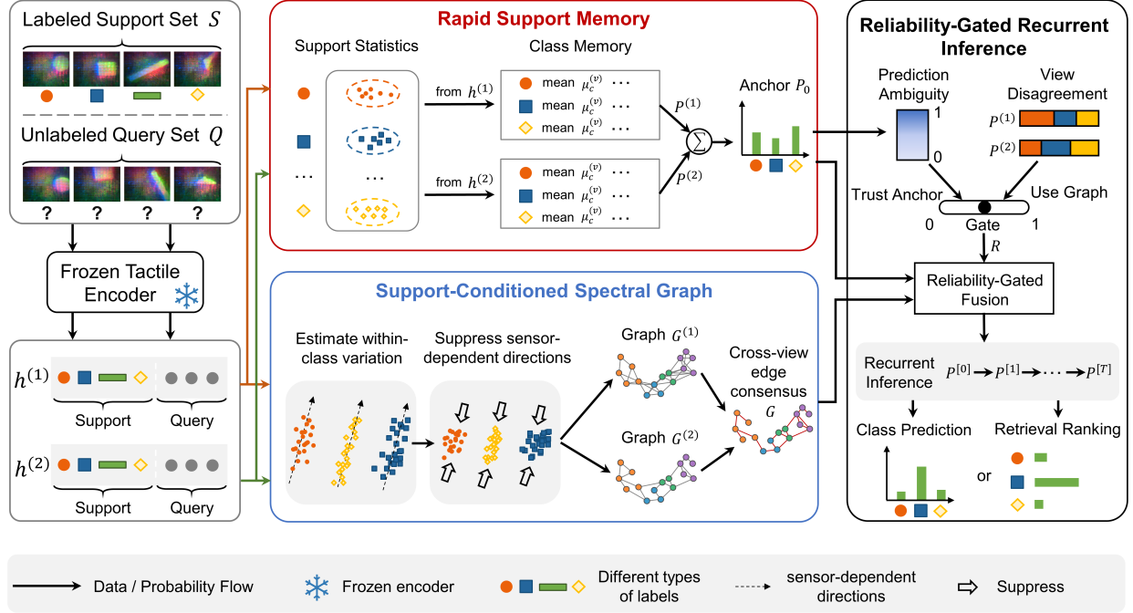
Figure 2: Information flow through BIFTA. A frozen encoder produces two readouts. Rapid support memory forms the probability anchor P_0 , while the support-conditioned spectral graph reshapes query geometry and constructs the cross-readout affinity matrix G . Prediction ambiguity and readout disagreement determine the query-wise reliability gate R . Anchored recurrent inference combines P_0 , G , and R to produce class probabilities or identity rankings.
