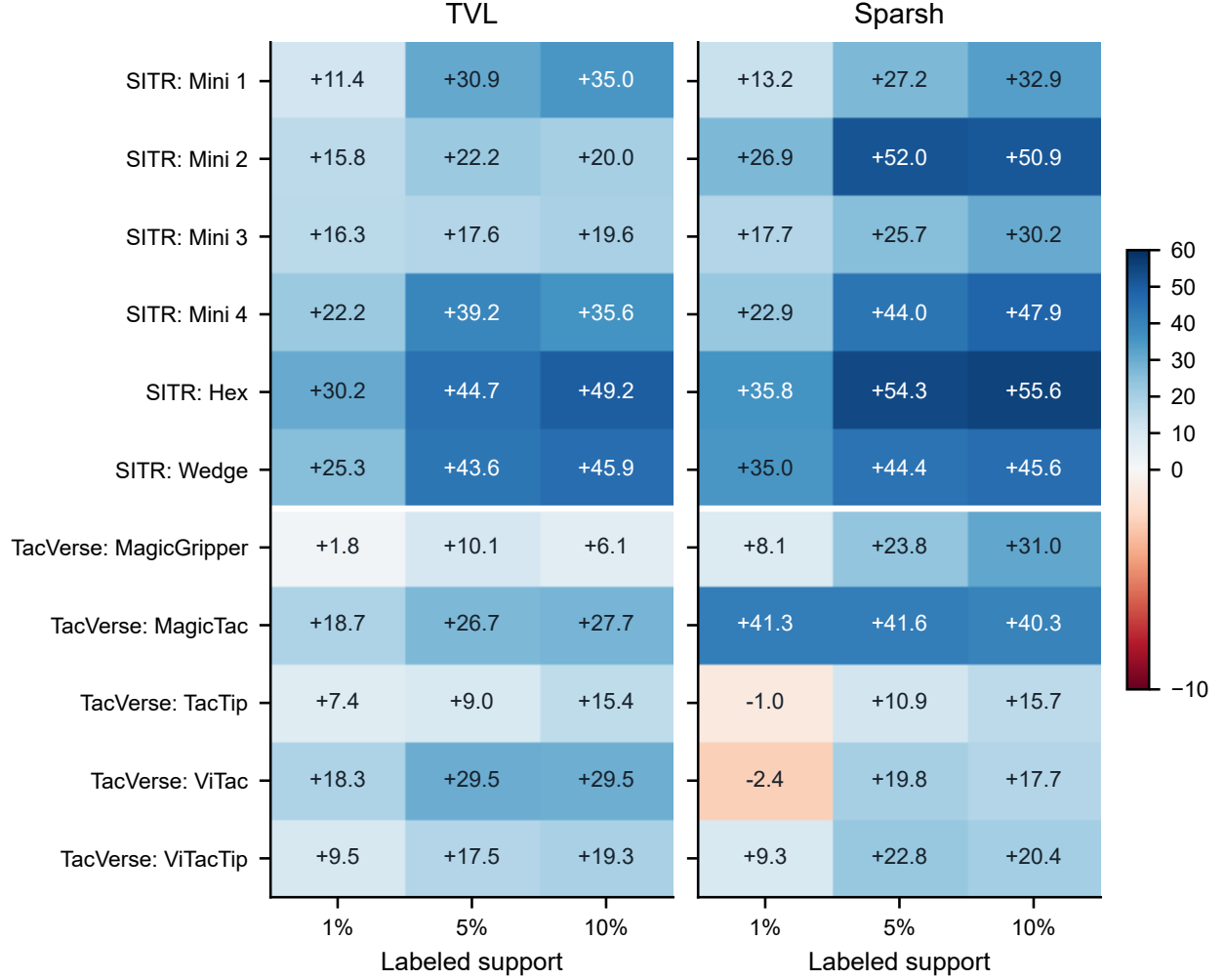
Figure 3: Performance comparison with the strongest baseline across sensors on SITR and TacVerse. Each cell reports the accuracy gain of BIFTA for the corresponding unknown sensor and label budget.
