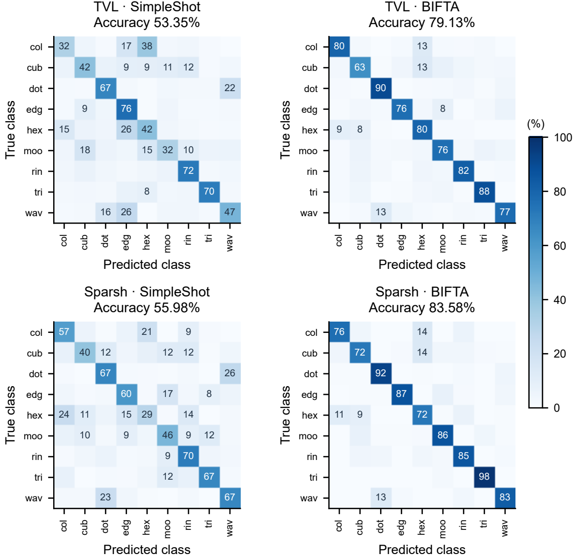
Figure 4: TacVerse class predictions with 10% support. Row-normalized confusion matrices compare SimpleShot and BIFTA on identical queries. Each matrix aggregates 13,500 predictions from five target sensors, three random seeds, and 900 queries per target.
