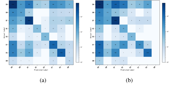
Fig. 4: Confusion matrix of (a) LingLan-14B (b) BianCang-14B-Instruct
