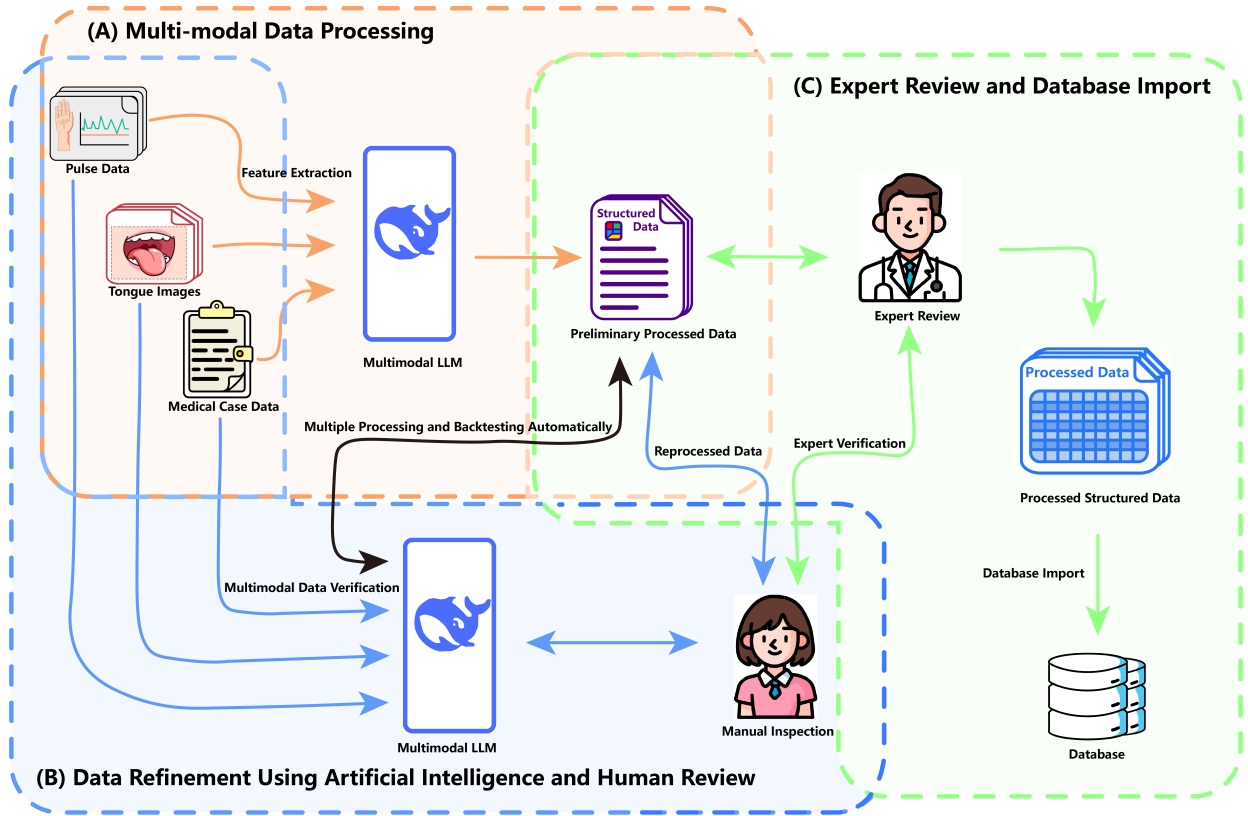
Fig. 2: An overview of UFMD: (A) Extract features from multimodal data via MLLM templates. (B) Refine data through MLLM review and expert validation. (C) Store verified structured data in persistent database.
