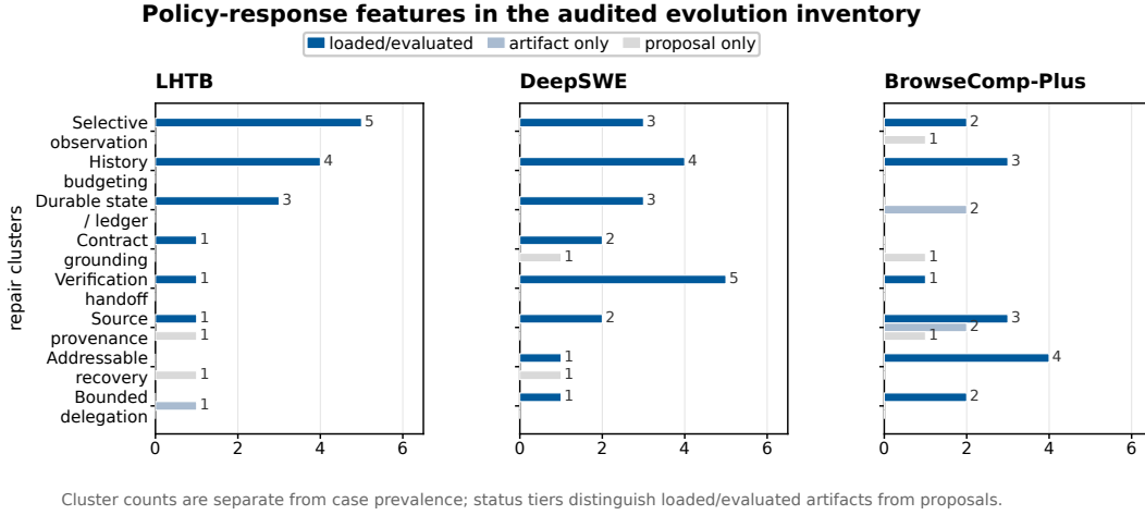
Figure 6: Repair-feature inventory by implementation status. Bars count deduplicated repair clusters in the audited policy artifacts, grouped by response feature and benchmark. “Loaded/evaluated” means the feature is present in a configured evaluated bundle; it does not establish that the feature fired or caused a reward change. Artifact-only and proposal-only items are shown separately. This inventory complements the case-prevalence figure in Section 6.3; the generic bulk/repeated-output problem label is not counted as a repair feature.
