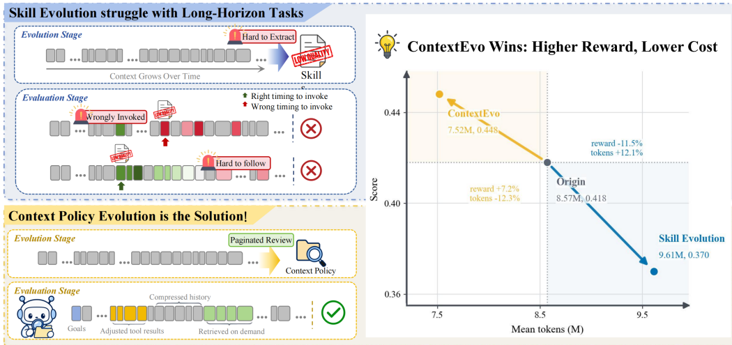
Figure 1: From skill evolution to context-policy evolution. As interaction histories grow, skill evolution may fail at both stages: extracting low-quality skills during evolution and invoking them at the wrong time or following them unreliably during evaluation. In contrast, our CONTEXTEVO evolves an efficient context policy, achieving higher scores with fewer tokens.
