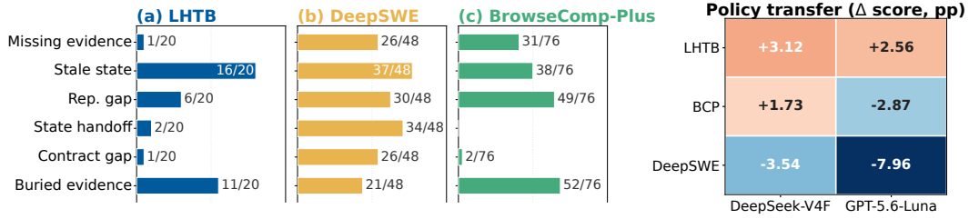
Figure 3: Environment-specific context problems and policy transfer. Bars show the share of audited cases with each multi-select context problem; labels report counts. The heatmap shows signed score changes (percentage points) from applying the LHTB-evolved policy under DeepSeek and Luna.
