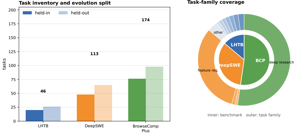
Figure 4: Benchmark coverage. The left panel reports the full inventory and the held-in/held-out split. The sunburst shows the benchmark inventory in the inner ring and task-family composition in the outer ring. LHTB shows its seven largest categories plus an “other” bucket, DeepSWE shows request types, and BrowseComp-Plus is a uniform multi-hop deep-research setting.
