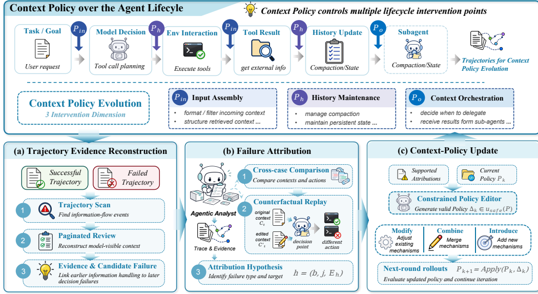
Figure 2: The overview of CONTEXTEVO. The context policy governs how information is presented, organized, and shared through the agent harness while the base model remains fixed. CONTEXTEVO reconstructs trajectory evidence, attributes context-management failures to policy dimensions, and applies constrained updates for the next evolution round.
