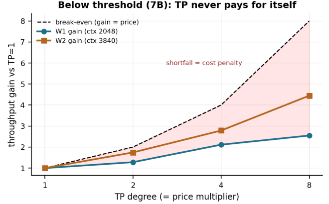
Fig. 5: Throughput gain against device-count price on Llama-2-7B S . The dashed line is break-even. Both workloads sit below it at every degree, so cost per token rises monotonically with tensor-parallel degree below the feasibility threshold . Sec. V-C shows this does not hold above it.
