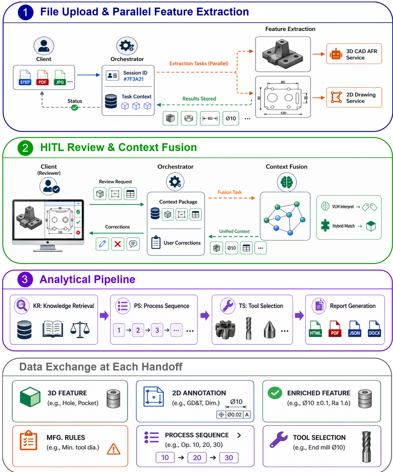
Fig. 2. End-to-end workflow of the proposed system, including file upload, parallel feature extraction, HITL review, context fusion, and downstream planning using progressively enriched design representations.
