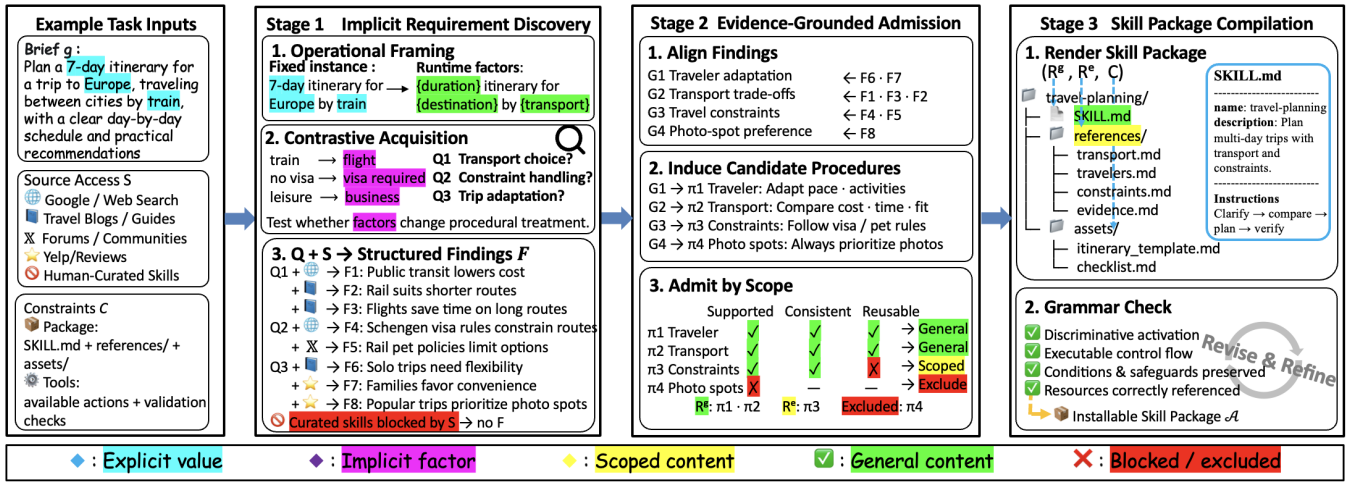
Figure 3: Overview of SKILLALCHEMY: \Phi_1 converts an underspecified brief into focused questions and structured findings, \Phi_2 induces candidate procedures and admits them via the evidence-supported scope, and \Phi_3 compiles the admitted content into an agent skill package.
