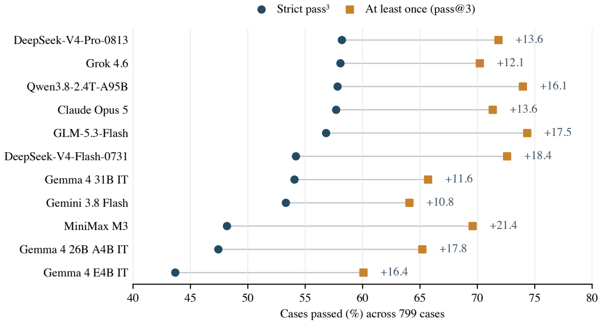
Figure 3: Strict reliability differs materially from at-least-once success. For every model, at-least-once success (pass@3) exceeds strict pass 3 (success on all three trials) by 10.8–21.4 percentage points over the released 799-case benchmark.
