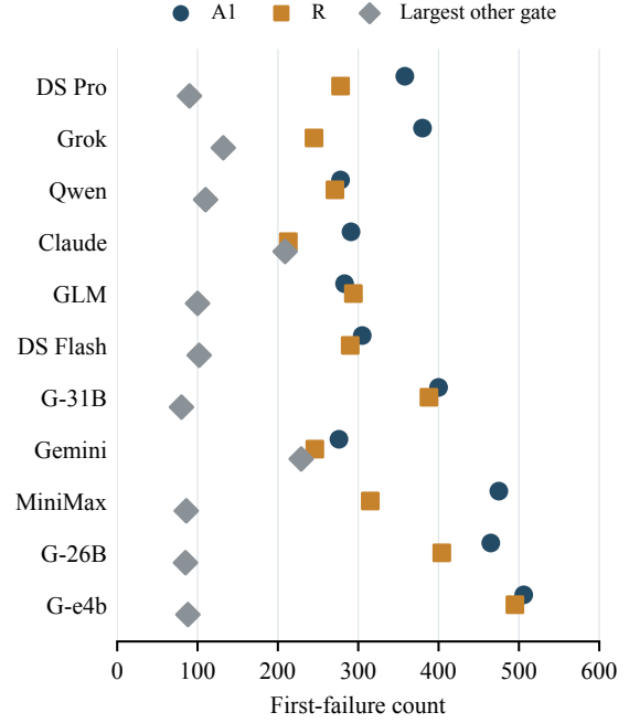
Figure 4: First-failure counts across all three passes. For every model, A1 (a required tool was not called) and R (the response missed its case-specific requirement) are the two largest first-failure gates. Complete counts appear in Table 10.
