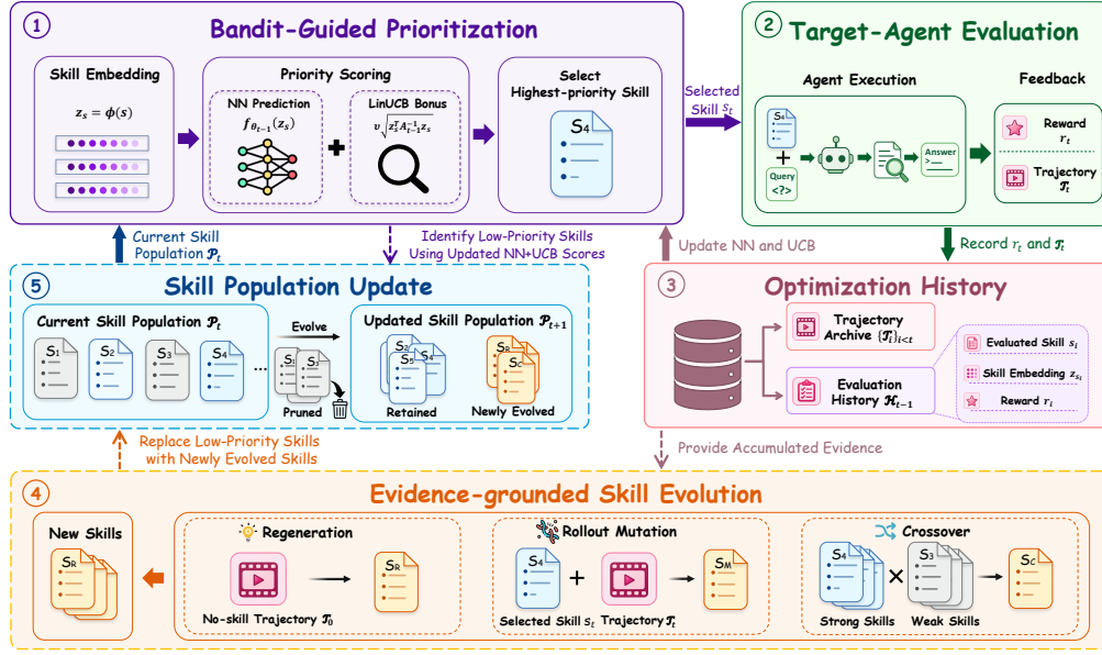
Figure 1: Overview of COBRA-Skills. At each round, skills in \mathcal{P}_t are prioritized using a neural reward predictor and LinearUCB bonus based on \mathcal{H}_{t-1} (①), and the highest-priority skill is evaluated by the target agent (②). The resulting reward and trajectories update the optimization history and scoring model (③). At scheduled population updates (performed periodically rather than after every round), new skills are evolved from accumulated evidence (④), and the updated priority scores from ① identify low-priority skills, which are replaced by the newly evolved skills to form \mathcal{P}_{t+1} (⑤). Dashed borders and arrows indicate scheduled-only operations.
