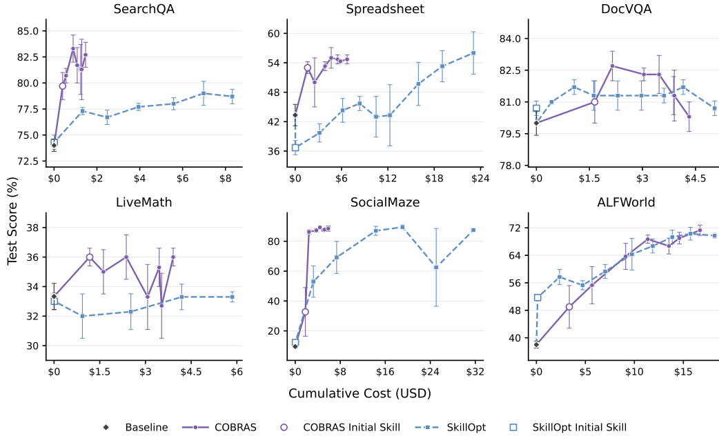
Figure 9: Checkpoint performance over cumulative optimization cost. Held-out test performance of the skill output by COBRA-Skills and SkillOpt at intermediate checkpoints, plotted against cumulative optimization cost across six benchmarks with Gemma4-26B-A4B-it as the target model.
