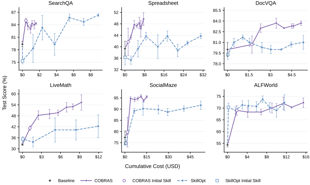
Figure 3: Checkpoint performance over cumulative optimization cost. Held-out test performance of the skill output by COBRA-Skills and SkillOpt at intermediate checkpoints, plotted against cumulative optimization cost across six benchmarks with Qwen3.6-35B-A3B as the target model.
