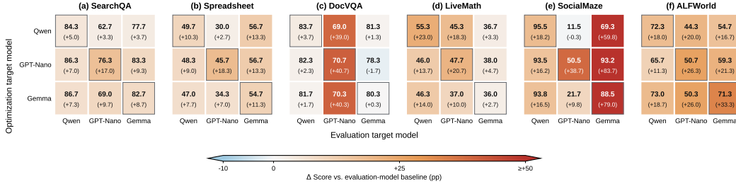
Figure 6: Cross-model transfer of optimized skills. Rows and columns denote the optimization and evaluation target models, respectively. Each cell reports the test score and the gain over the evaluation model’s no-skill baseline; outlined cells indicate in-model evaluation. GPT-5.5 is used as the teaching model throughout.
