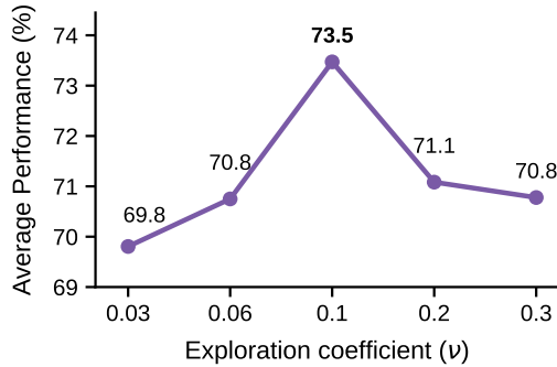
Figure 7: Sensitivity of COBRA-Skills to the LinearUCB exploration coefficient \nu on Qwen3.6-35B-A3B, averaged across the six benchmarks.
