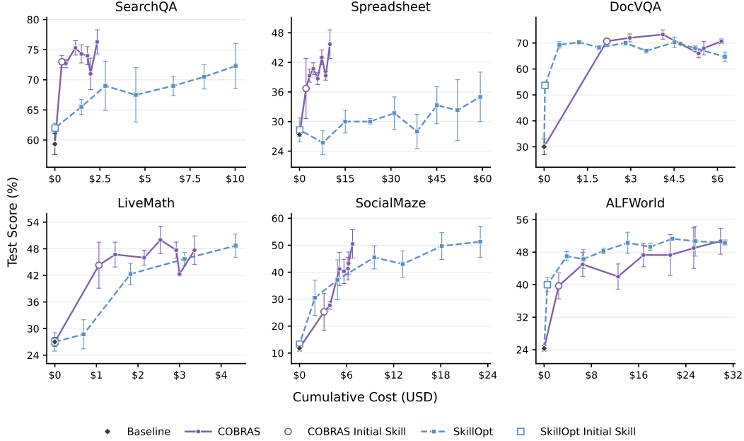
Figure 8: Checkpoint performance over cumulative optimization cost. Held-out test performance of the skill output by COBRA-Skills and SkillOpt at intermediate checkpoints, plotted against cumulative optimization cost across six benchmarks with GPT-5.4-Nano as the target model.
