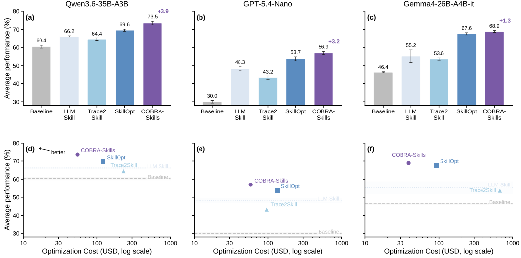
Figure 2: Overall performance and cost-effectiveness across target models. Top: average test performance across six benchmarks for three target models. Bottom: the relationship between average test performance and total optimization cost under the native harness.
