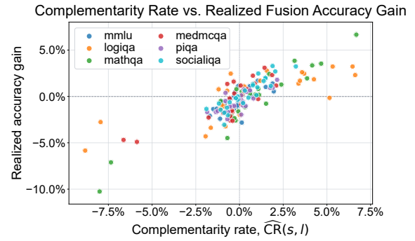
Figure 5: Calibration-set complementarity rate versus realized accuracy gain from confidence-weighted fusion over direct deferral. Each point represents one dataset-model-pair evaluation across six LLM tasks; dashed lines indicate zero complementarity and zero gain.
