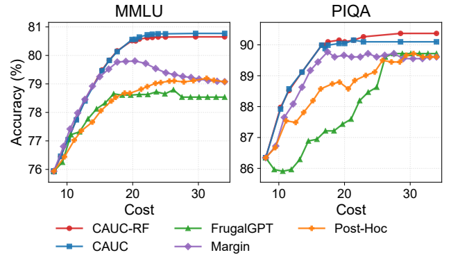
Figure 3: Accuracy–cost trade-offs across operating points on MMLU and PIQA.
