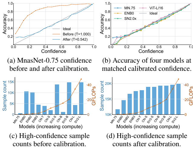
Figure 4: Calibration reliability and high-confidence coverage on ImageNet. High-confidence counts use [0.85, 1.00] , and the orange curve denotes model GFLOPs.
