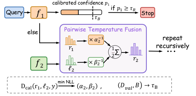
Figure 2: CAUC-RF recursively fuses calibrated outputs using learned pairwise temperatures and applies a shared confidence threshold for early stopping.
