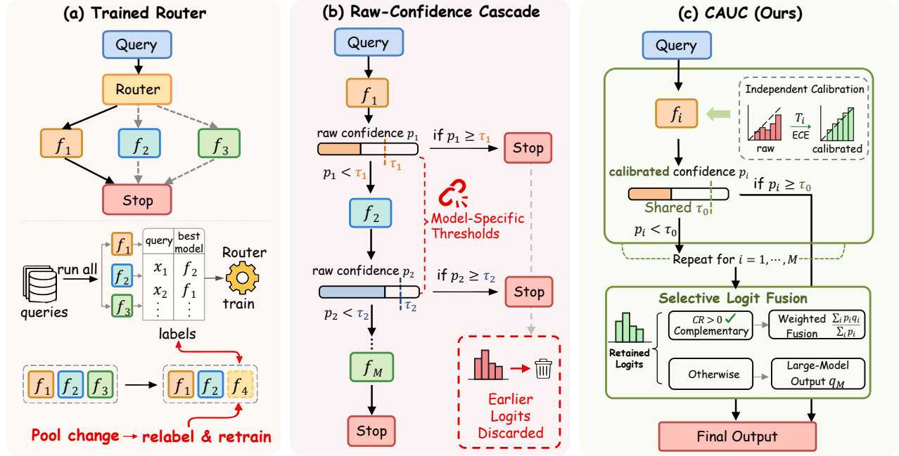
Figure 1: Comparison of collaboration paradigms for heterogeneous models. (a) Trained routers need labeled routing data and retraining after model-pool changes. (b) Raw-confidence cascades use model-specific thresholds and discard earlier predictions upon deferral. (c) CAUC independently calibrates models to enable a shared threshold across the cascade. It selectively fuses retained logits when they are complementary; otherwise, it uses the final model’s prediction.
