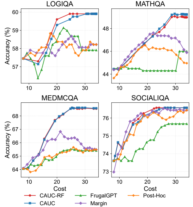
Figure A1: Two-model accuracy–cost trade-offs for Ministral-3-8B → Gemma-4-26B across operating points on LogiQA, MathQA, MedMCQA, and SocialIQA, complementing the MMLU and PIQA results reported in the main paper.
